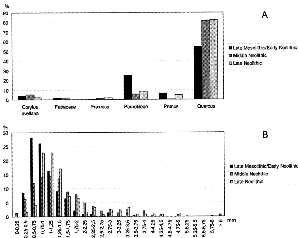
A - Synthetic percentage charcoal diagram for twelve sites of southern littoral of Brittany (France)
