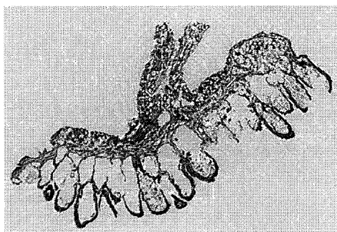
SRXTM images of charcoalified pteridosperm pollen organ from the Mississippian (Carboniferous) of Scotland.
