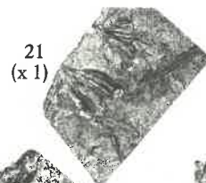
20 - 21. cf. Calathiops sp.
