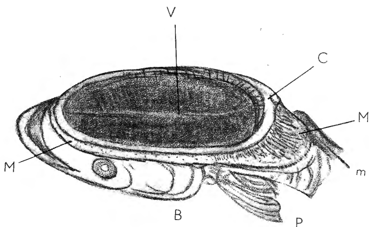
Fig. 3. — Echeneis (spec. ?) × 2.
