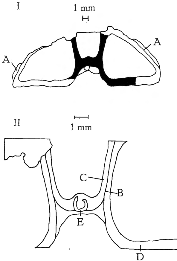
Fig. 13. — Syringothyris sp.
