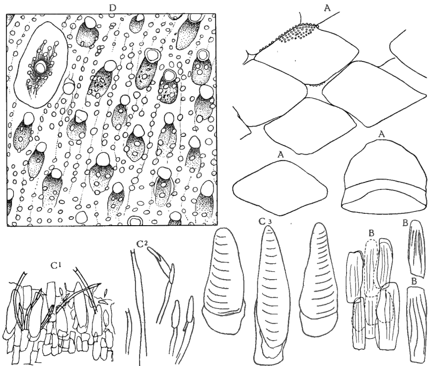
Fig. 3. — Chiton peregrinus THEILE, 1910. Karachi.
