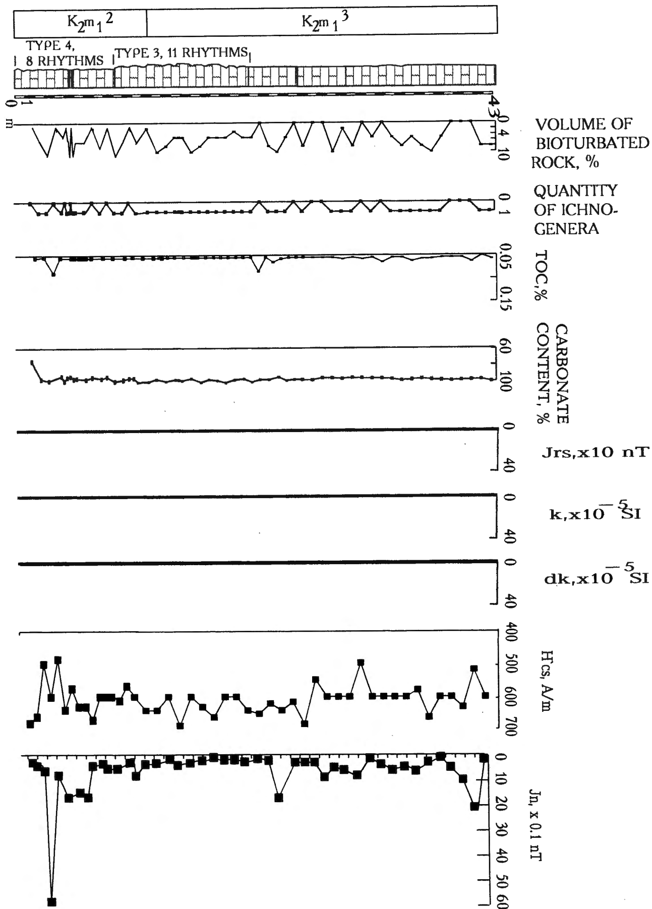
Text-fig. 6 — Lower Maastrichtian of Volsk section, Ulyanovsk-Saratov foredeep. Explanation of signatures used in Text-fig. 2.
