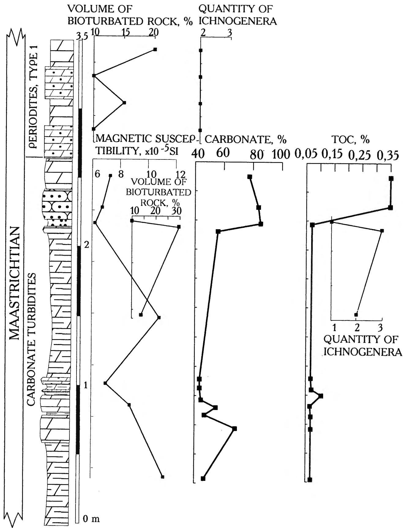
Text-fig. 3 — Maastrichtian transitional turbidite-periodite succession of Betta section, Caucasus. Explanation of signatures used in Text-fig. 2.
