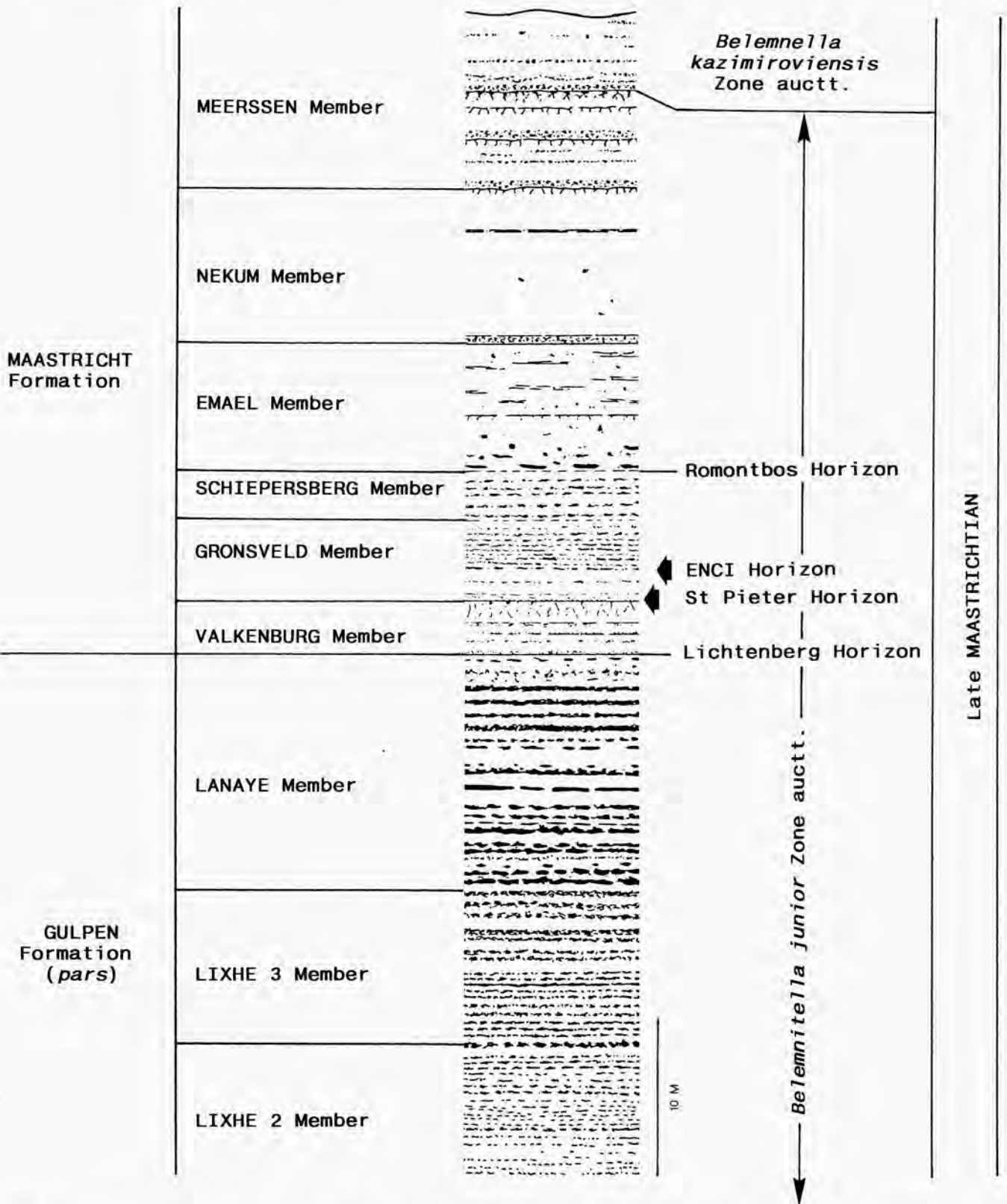
Fig. 2 — Lithostratigraphy (modified after FELDER et al. , 1978), coleoid cephalopod biozones and chronostratigraphy of the section exposed at the ENCI Nederland BV quarry (Maastricht); the arrows mark the provenance of the material of Dunnicrinus aequalis (D'ORBIGNY, 1841) described in the present paper.
