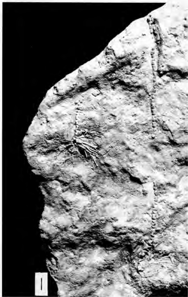
Fig. 3 – Two pluricolumnals with radicular attachment structures of Dunicrinus aequalis (D'ORBIGNY, 1841) on a slab (NHMM RD 229) from the base of the Gronsveld Member, ENCI Nederland BV quarry (Maas-tricht); scale bar equals 10 mm.
