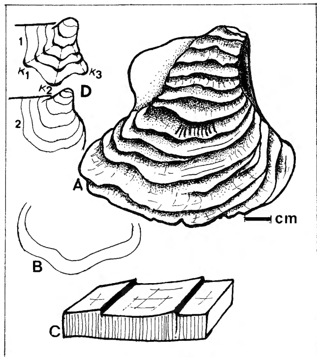
Text-fig. 4 — A - Inoceramus (Volviceramus) cf. koeneni G. MÜLLER, from Lonzée. B - Shape of the undulations of I. (Volviceramus) cf. koeneni G. MÜLLER. C - Shell structure of I. (Volviceramus) cf. koeneni G. MÜLLER. D - 1: I. (Cordiceramus) cordiformis J. de C. SOWERBY (k1, k2, k3 corners); 2: I. (Volviceramus) koeneni G. MÜLLER.
