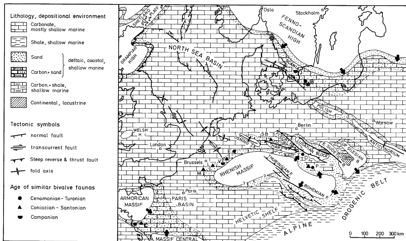
Text-fig. 3 — Palaeogeographical map for the Senonian-Danian of central Europe (after ZIEGLER, 1990). B - Bornholm; C - Commequiers; D - Dresden; E - Essen/Ruhr; J - Ifö; L - Lonzé; M - Mons; P - Prague; SB - Subhercynian Basin; V - Vaals.
