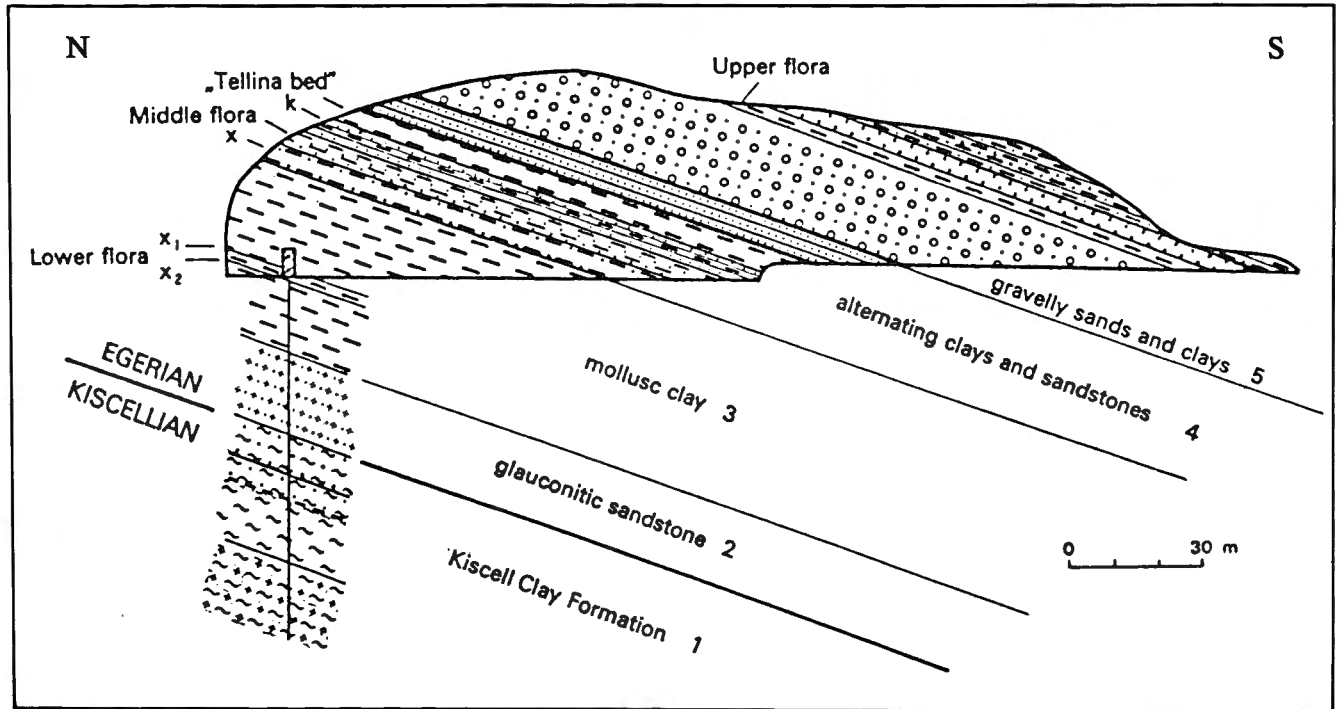
Fig. 3 — Section of the Wind brickyard at Eger, holostratotype of the regional Egerian stage (from BALDI-BEKE, 1989a).
