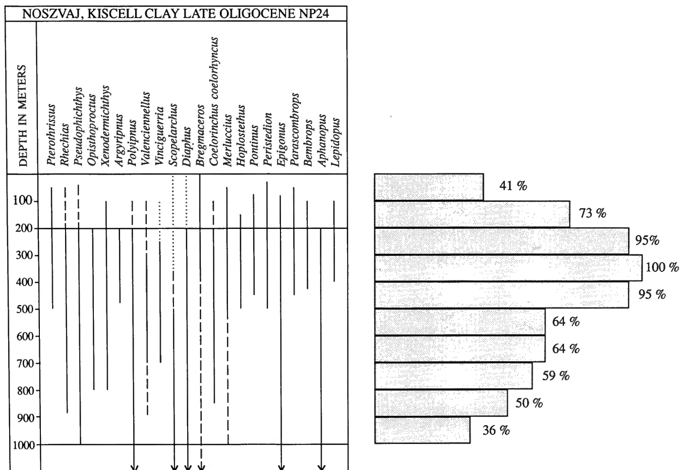
Fig. 6 — Recent bathymetric distribution of teleost taxa represented in the Kiscell Clay at Noszvaj; dotted lines represent nightly presence of some mesopelagic species at the surface and interrupted lines represent less regular presence at the corresponding depth. See main text for explanation of methodology, and see NOLF & BRZOBHATY (1993) for bibliographic references on bathymetric distribution of Recent fishes.
