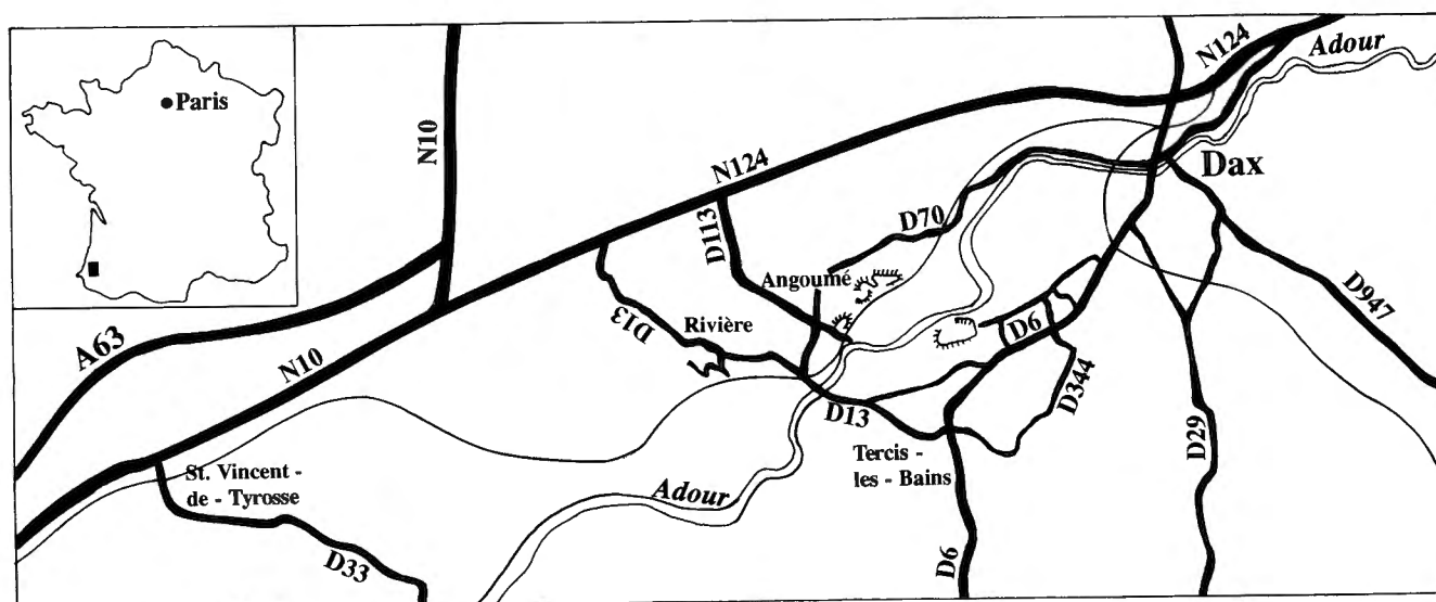
Fig. 1 — Location of "La Grande Carrière", Tercis, Landes.
