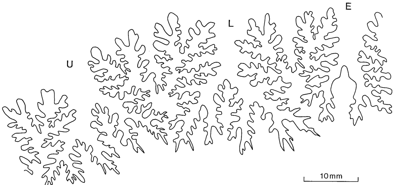
Fig. 9. Suture line of Diplomoceras cylindraceum (DEFRANCE, 1816). Based on IRSNB 10257 (IG 6521). Bar scale is 10 mm.
