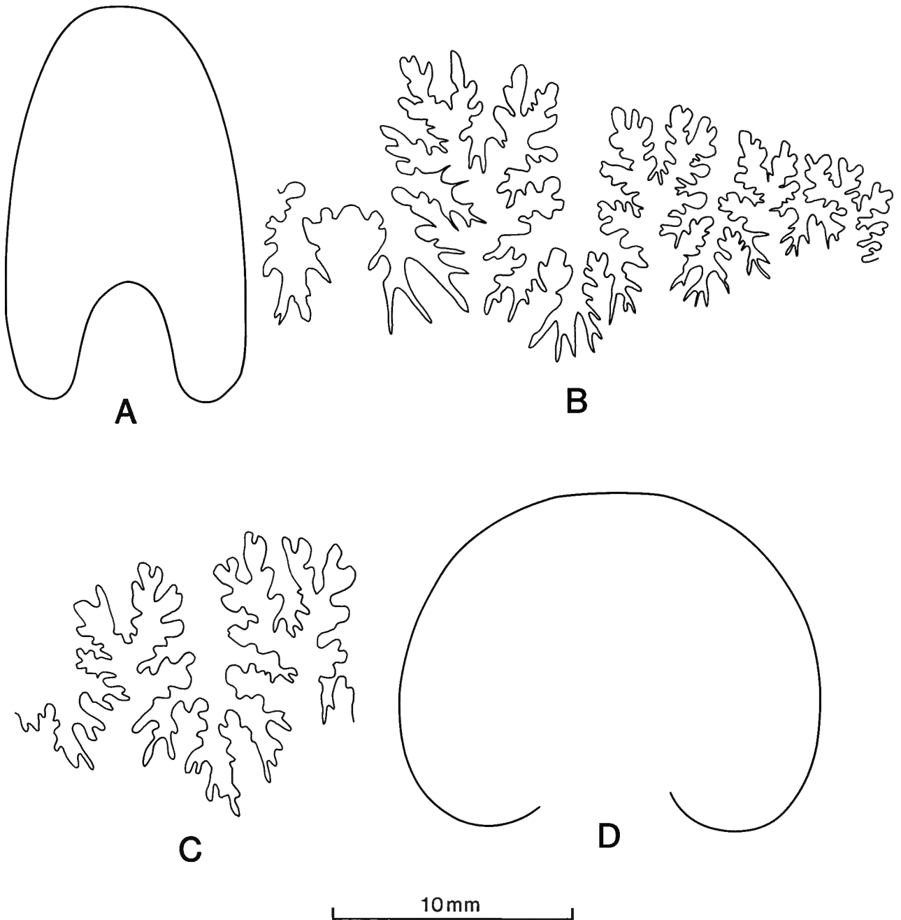
Fig. 7. External sutures and whorl sections of: A, C, Pachydiscus ( Pachydiscus ) gollevillensis (d'ORBIGNY, 1850) IRSNB 9476; B, Pachydiscus ( Pachydiscus ) jacquoti SEUNES, 1890 IRSNB 9481; D, Saghalinites sp. IRSNB IG 6521. Bar scale is 10 mm.
