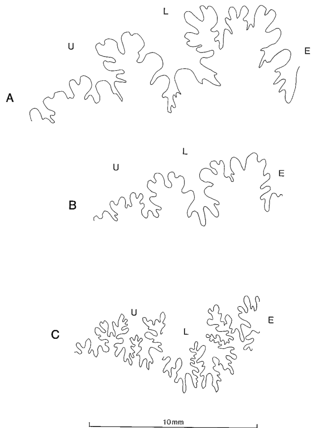
Fig. 13. External sutures of: A, B, Hoploscaphites constrictus (J. SOWERBY, 1817) based on A, NMM MK 2874; B, NMM MK 734; C, Hoploscaphites felderi sp. nov. based on BMNH C75619. Bar scale is 10 mm.
