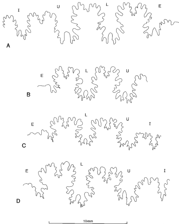
Fig. 11. Suture lines of: A, B, Baculites vertebralis LAMARCK, 1801 based on A, IRSNB 10278 (IG 6521); B, IRSNB 10258 (IG 6521). C, D, Baculites anceps LAMARCK, 1822 based on C, SMC F2823; D, SMC F2822. Bar scale is 10 mm.
