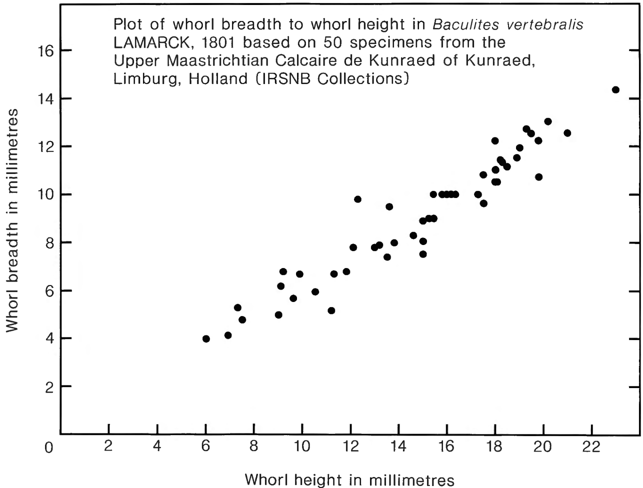
Fig. 12. Scatter plot of whorl breadth versus whorl height in Baculites vertebralis LAMARCK, 1801.
