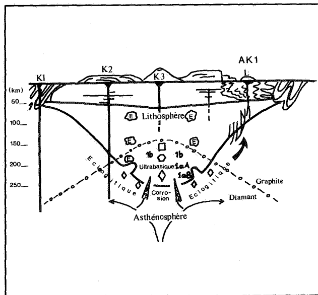
Figure 3 : Haggerty's structural model (1986) relating the kimberlitic and lamproitic intrusions and the craton.
