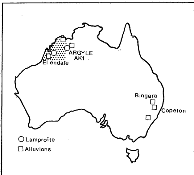
Figure 1 : Map of Australia indicating the most important diamond deposits. The dotted area indicates the position of the Kimberley "craton" in Western Australia.
