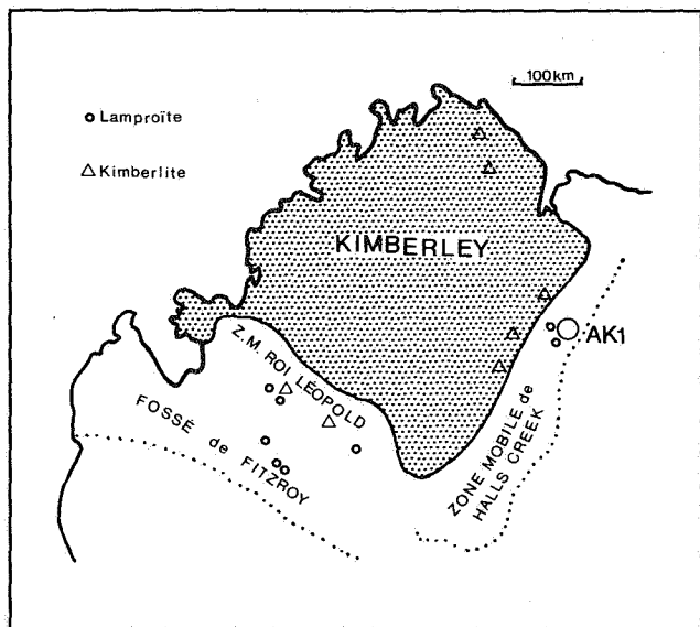
Figure 2 : Map showing the geological structure of the northern part of Western Australia. The dotted area represents the Kimberley Craton with adjacent the King Leopold' and the Halls Creek Mobile Belt.
