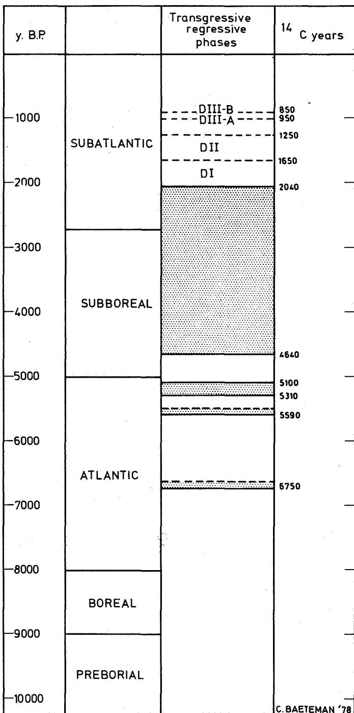
Fig. 2. - Chronological timescale.
