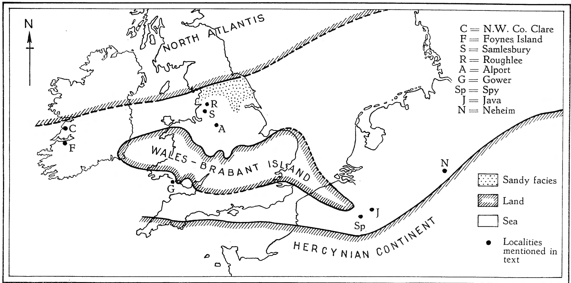
TEXT FIG. 2. — Palaeogeographical map of North-West Europe during the Homoceras Age with the location of places mentioned in the text.
