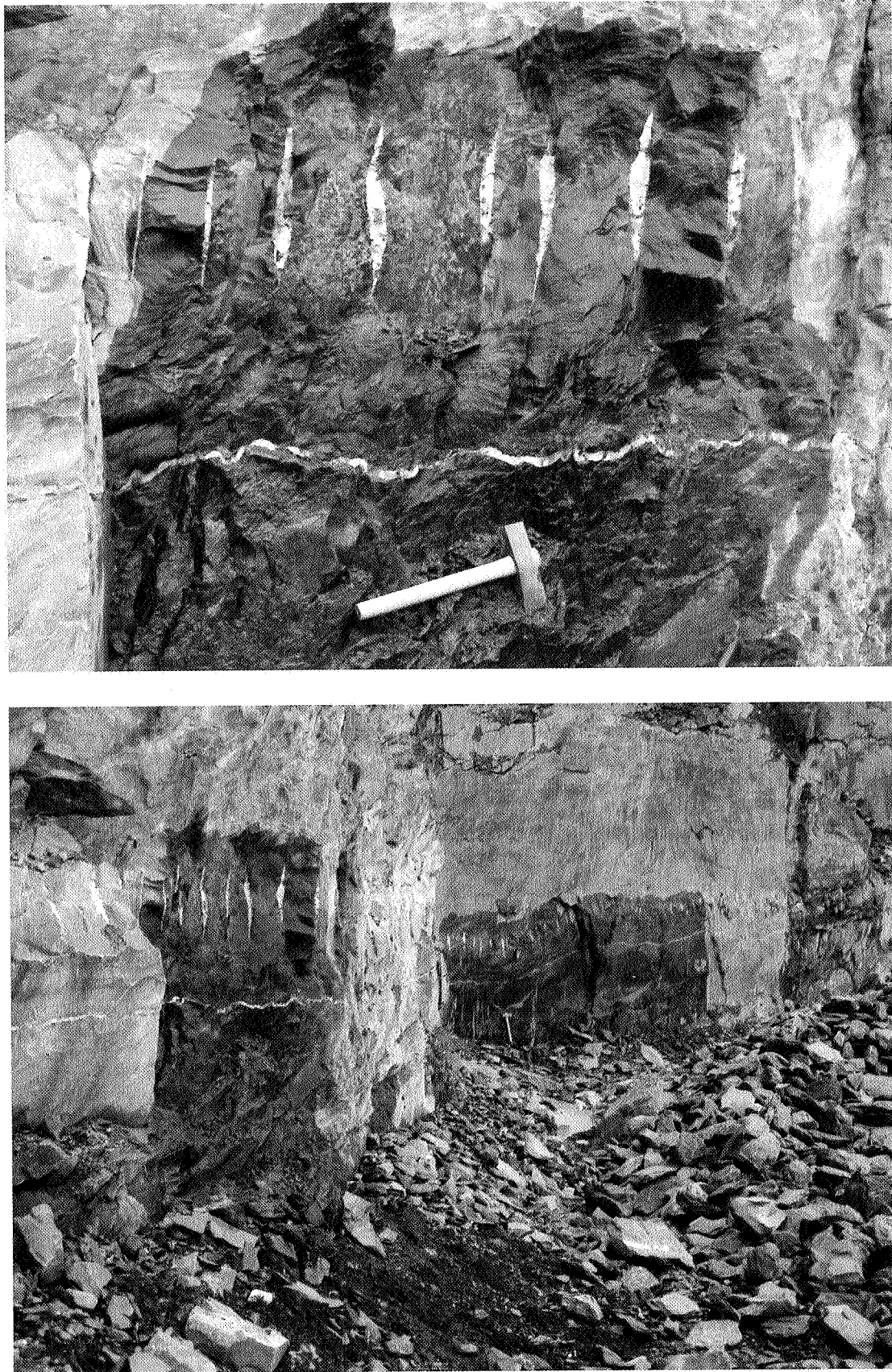
Figure 7.23 Association of lens-shaped quartz veins normal to the bedding plane and a layer-parallel quartz vein slightly folded.
