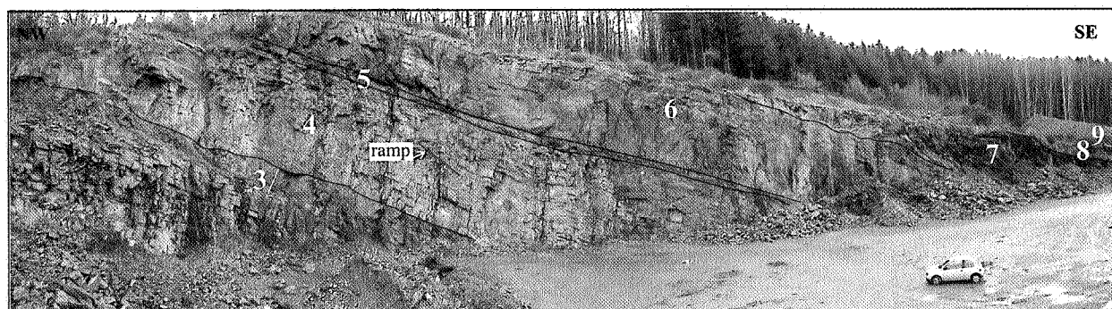
Figure 7.8 Main face of the Lambert Quarry. White numbers refer to the various sedimentary units as defined by Goemaere and Dejonghe (2005). See text for details.
