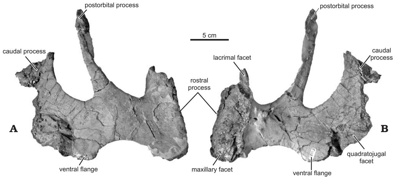
Fig. 7. Right jugal of hadrosaurid dinosaur Olorotitan arharensis Godefroit, Bolotsky, and Alifanov 2003 (AEHM 2/845, holotype), from the Upper Cretaceous of Kundur (Russia), in lateral (A) and medial (B) views.
