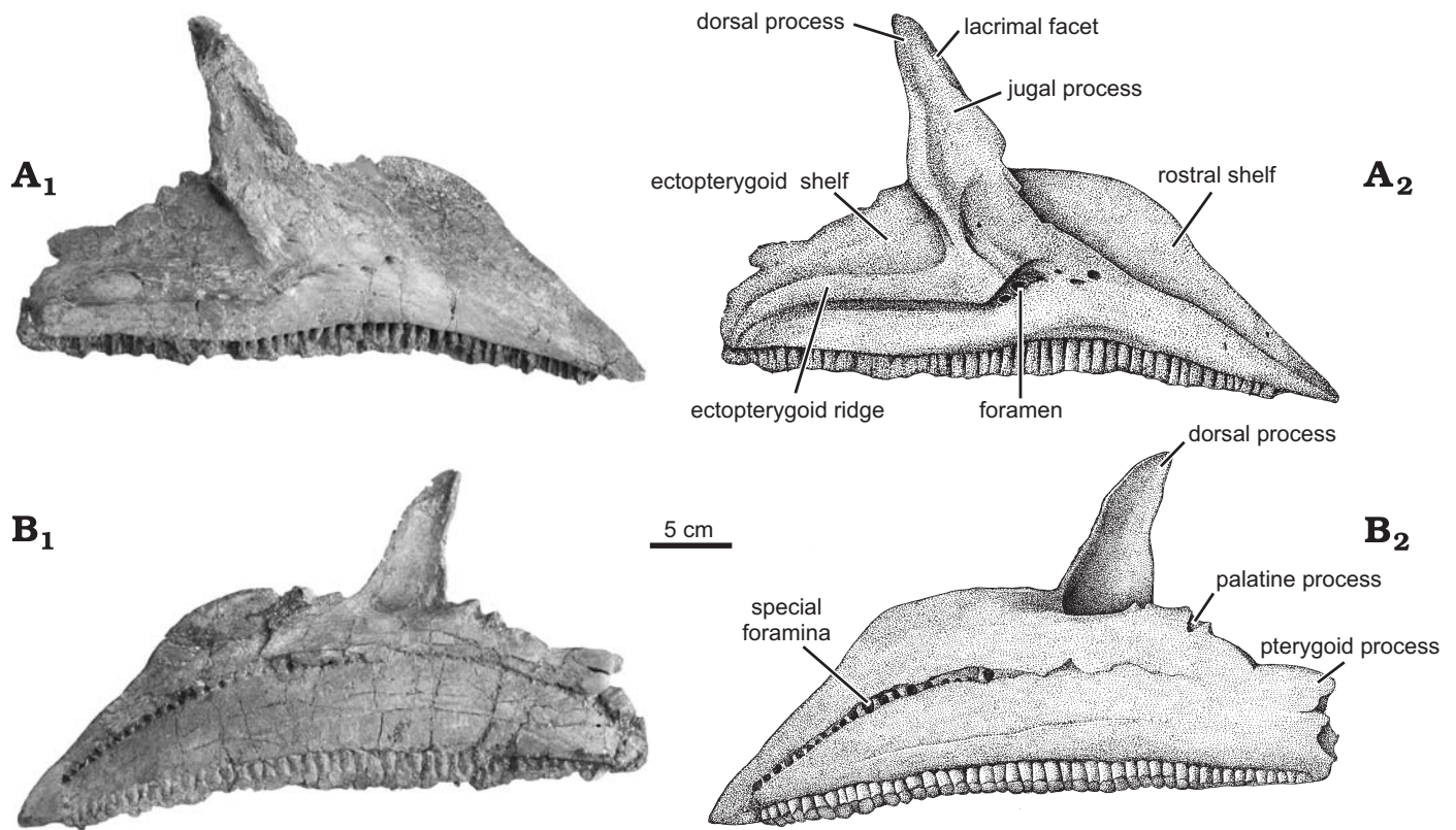
Fig. 6. Right maxilla of hadrosaurid dinosaur Olorotitan arharensis Godefroit, Bolotsky, and Alifanov 2003 (AEHM 2/845, holotype), from the Upper Cretaceous of Kundur (Russia), in lateral (A) and medial (B) views. Photographs (A 1 , B 1 ), explanatory drawings (A 2 , B 2 ).
