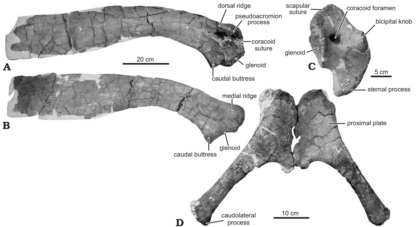
Fig. 18. Hadrosaurid dinosaur Olorotitan arharensis Godefroit, Bolotsky, and Alifanov 2003 (AEHM 2/495, holotype), from the Upper Cretaceous of Kundur (Russia). A. Right scapula, in lateral view. B. Left scapula, in medial view. C. Right coracoid, in lateral view. D. Sterna, in ventral view.
