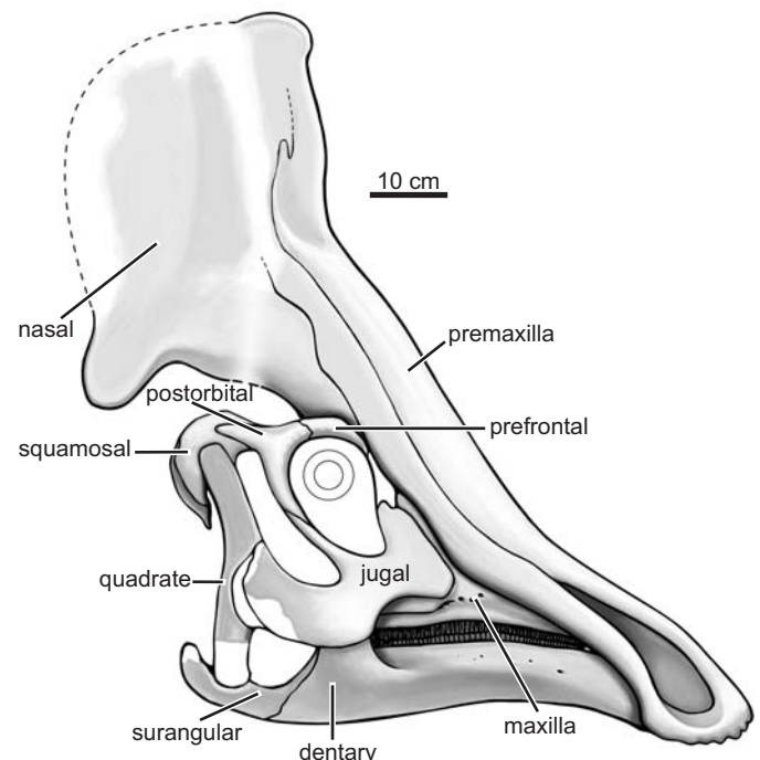
Fig. 3. Reconstruction of the skull of hadrosaurid dinosaur Olorotitan arharensis Godefroit, Bolotsky, and Alifanov 2003, from the Upper Cretaceous of Kundur (Russia), in right lateral view.
