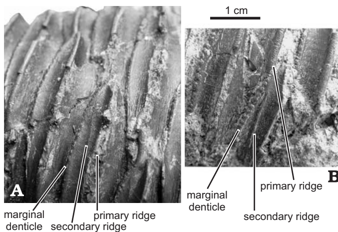
Fig. 11. Right dentary teeth of hadrosaurid dinosaur Olorotitan arharensis Godefroit, Bolotsky, and Alifanov 2003 (AEHM 2/845, holotype), from the Upper Cretaceous of Kundur (Russia), in lingual views. A. From the middle part of the dental battery. B. From the caudal part of the dental battery.
