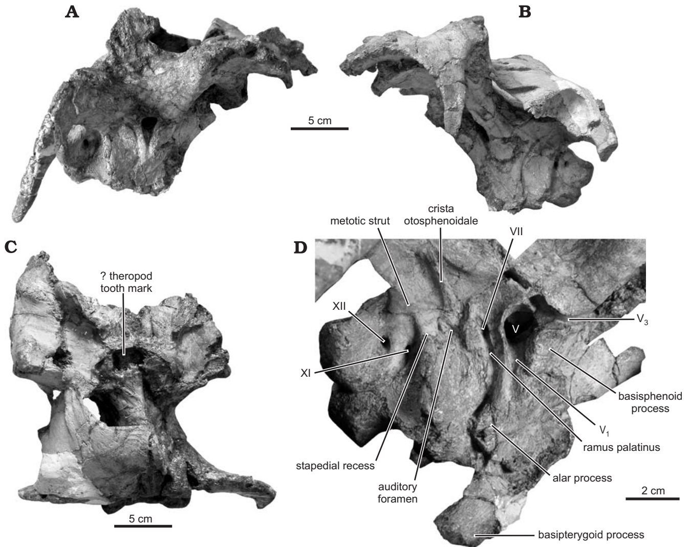
Fig. 5. Photographs of the braincase of hadrosaurid dinosaur Olorotitan arharensis Godefroit, Bolotsky, and Alifanov 2003 (AEHM 2/845, holotype), from the Upper Cretaceous of Kundur (Russia), in right lateral (A), left lateral (B), and dorsal (C) views. D. Details of the right lateral view of the braincase.
