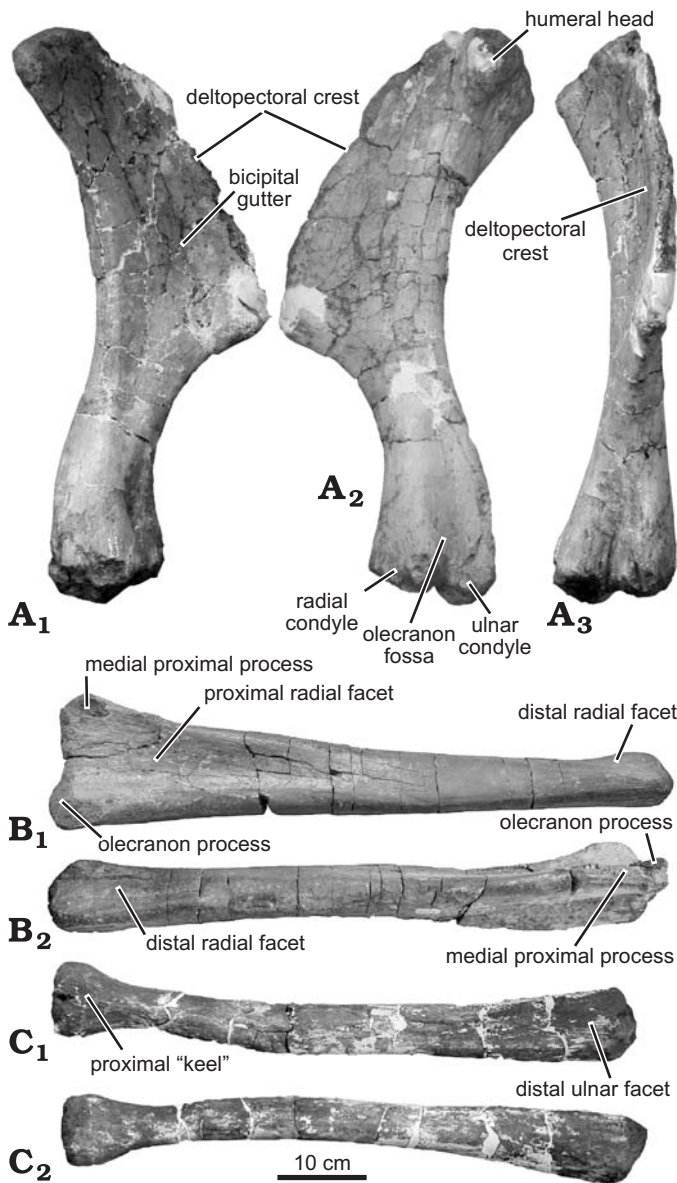
Fig. 19. Hadrosaurid dinosaur Olorotitan arharensis Godefroit, Bolotsky, and Alifanov 2003 (AEHM 2/845, holotype), from the Upper Cretaceous of Kundur (Russia). A. Left humerus, in cranial (A 1 ), caudal (A 2 ), and lateral (A 3 ) views. B. Right ulna, in cranial (B 1 ) and medial (B 2 ) views. C. Right radius, in caudal (C 1 ) and cranial (C 2 ) views.
