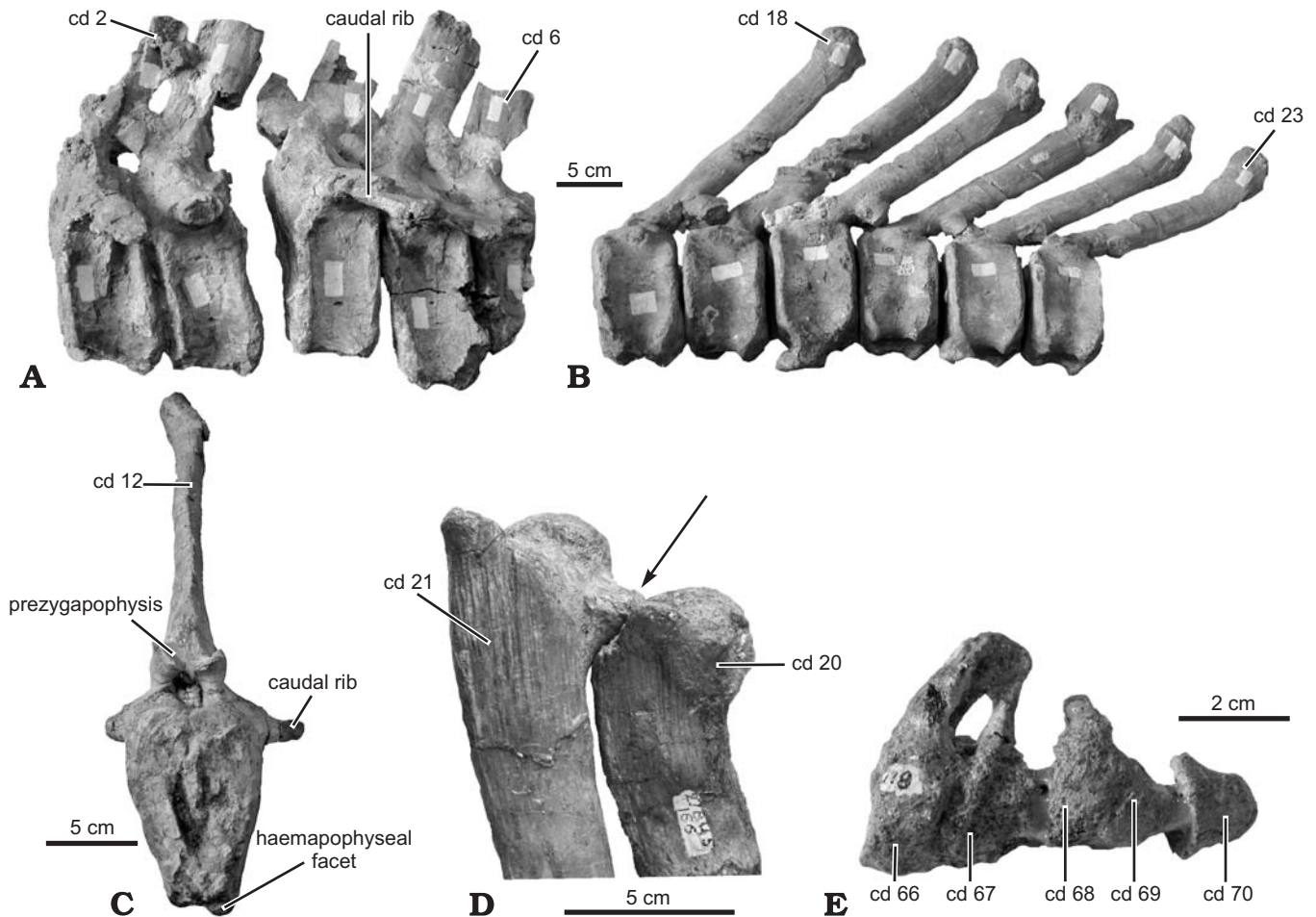
Fig. 17. Caudal vertebrae of hadrosaurid dinosaur Olorotitan arharensis Godefroit, Bolotsky, and Alifanov 2003 (AEHM 2/845, holotype), from the Upper Cretaceous of Kundur (Russia). A. Caudal vertebrae 2–6, in left lateral view. B. Caudal vertebrae 18–23, in left lateral view. C. Caudal vertebra 12, in cranial view. D. Supplementary articulation (indicated by an arrow) between the neural arches of caudal vertebrae 20–21. E. Caudal vertebrae 66–70, in left lateral view. cd, caudal vertebra.
