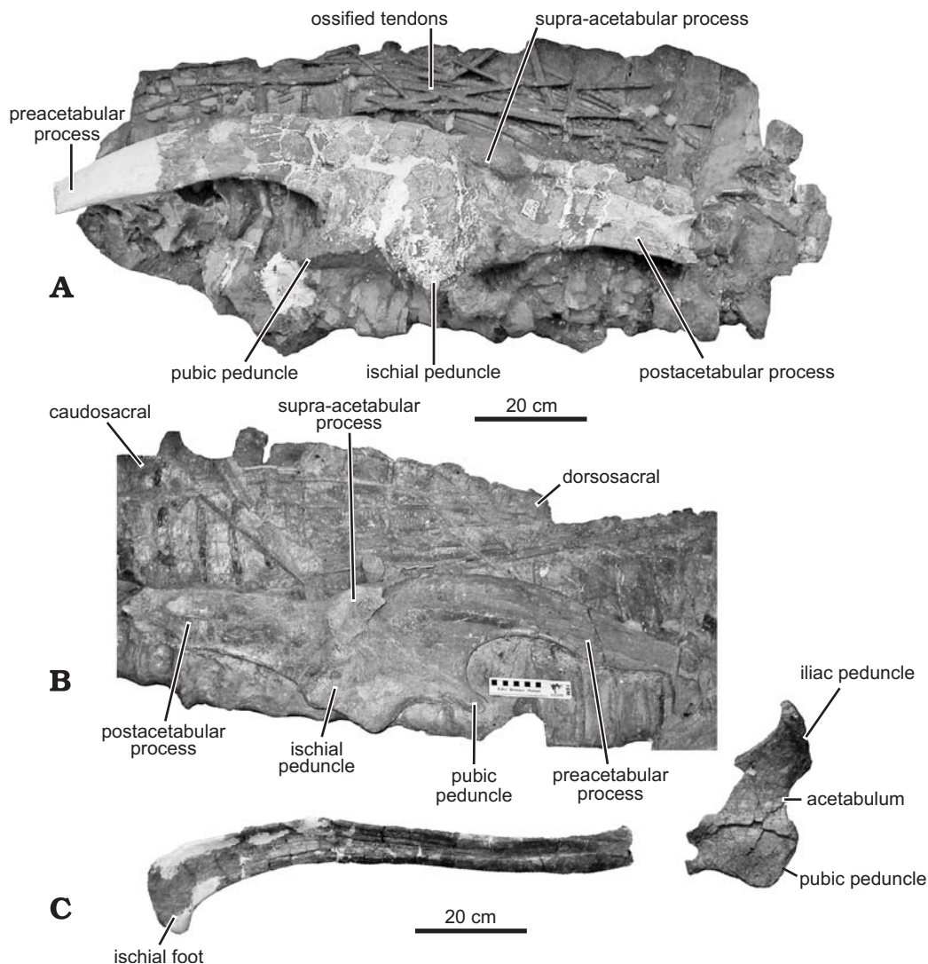
Fig. 16. Hadrosaurid dinosaur Olorotitan arharensis Godefroit, Bolotsky, and Alifanov 2003, from the Upper Cretaceous of Kundur (Russia). A. Sacral block and left ilium of AEHM 2/845 (holotype), in lateral view. B. Sacrum, caudal part of the dorsal vertebrae and right ilium of AEHM 2/846, in lateral view. C. Left ischium of AEHM 2/845 (holotype), in medial view.
