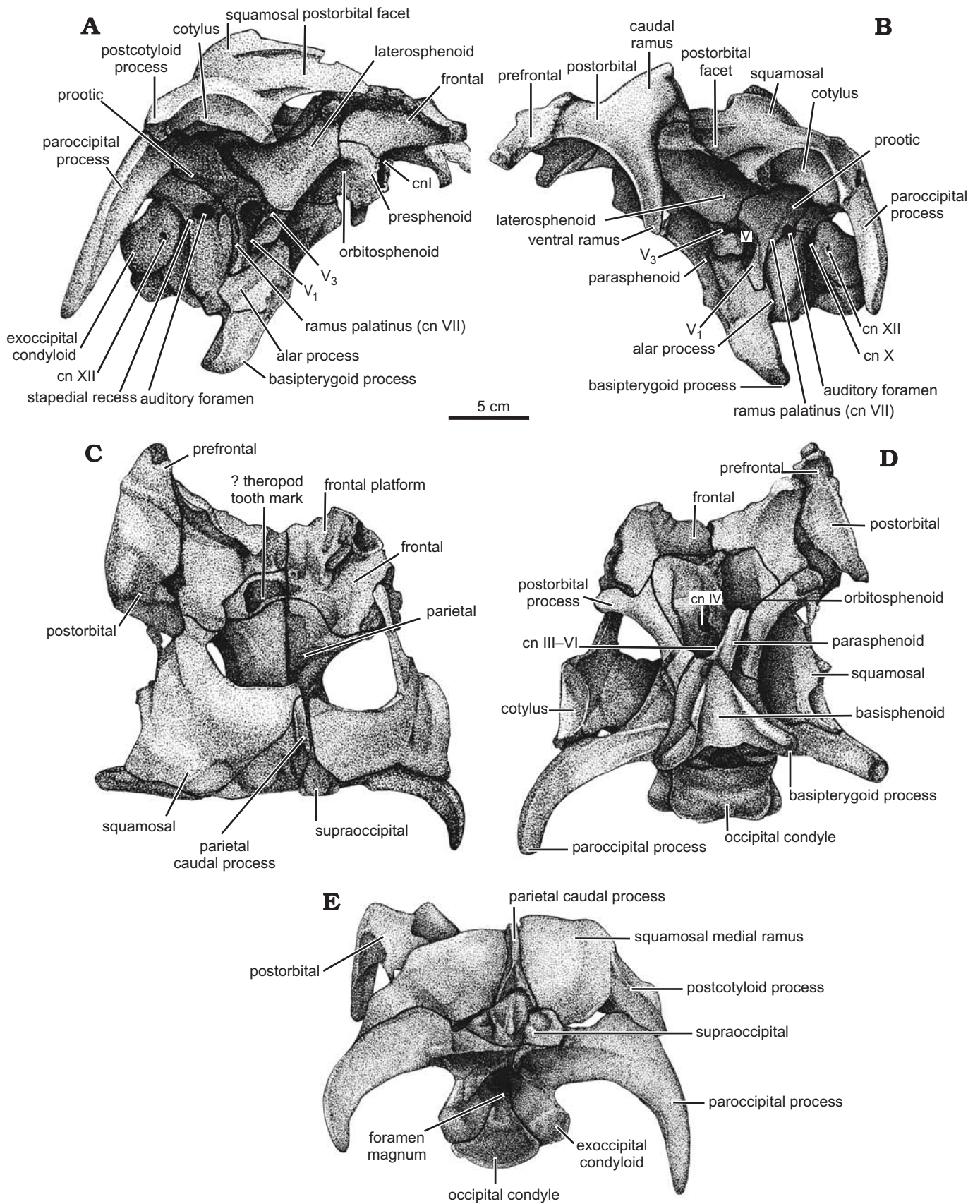
Fig. 4. Interpretative drawings of the braincase of hadrosaurid dinosaur Olorotitan arharensis Godefroit, Bolotsky, and Alifanov 2003 (AEHM 2/845, holotype), from the Upper Cretaceous of Kundur (Russia), in right lateral (A), left lateral (B), dorsal (C), ventral (D), and caudal (E) views. cn, foramina for cranial nerves.
