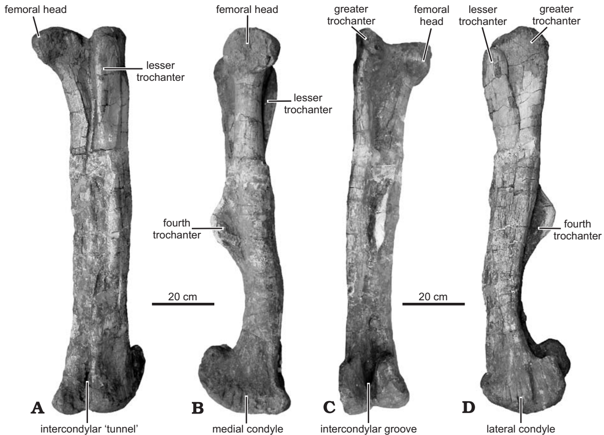
Fig. 20. Left femur of hadrosaurid dinosaur Olorotitan arharensis Godefroit, Bolotsky, and Alifanov 2003 (AEHM 2/845, holotype), from the Upper Cretaceous of Kundur (Russia), in cranial (A), medial (B), caudal (C), and lateral (D) views.
