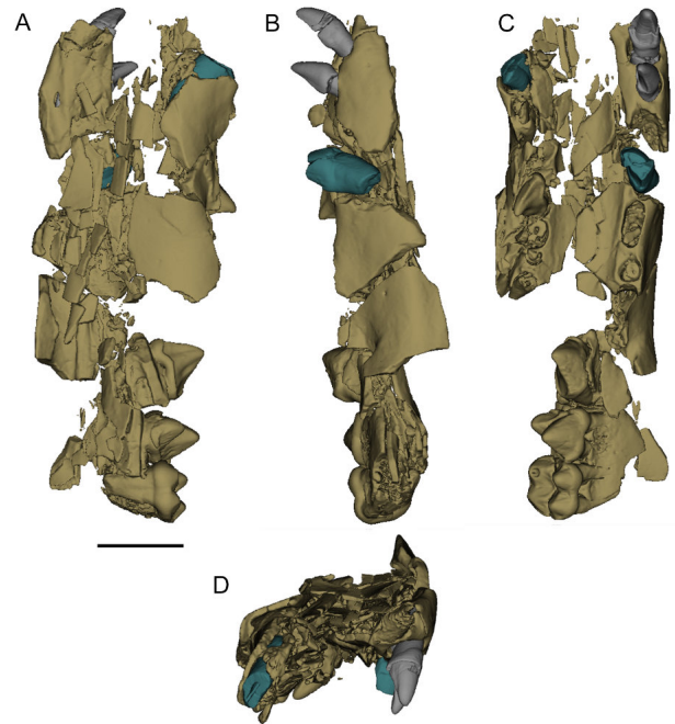
Figure 2. Illustration of the 3D model of GU/RJ/157 before restoration showing the breakage and main deformations, especially the shearing between right and left sides taking the canine as a hallmark (in blue) in A) dorsal, B) lateral, C) ventral, D) anterior views; the canines are highlighted in blue, incisors in grey. Scale bar = 1cm.
