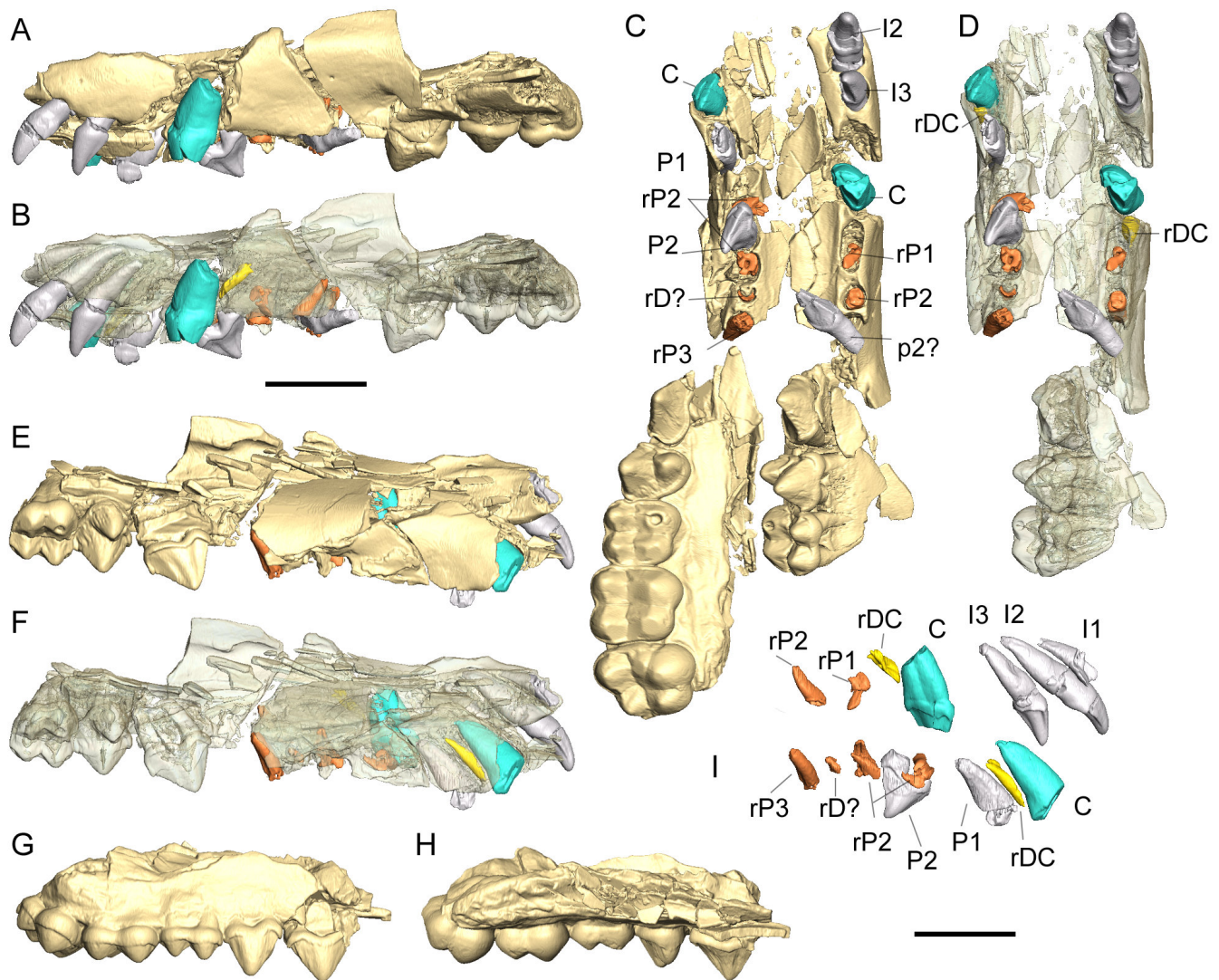
Figure 1. Illustration of the 3D model of GU/RJ/157 showing the preserved dentition in A-B) left lateral, C-D) ventral, E-F) right lateral, G-H) right and left lateral, I) right oblique (without bone) views; Abbreviations: r, root; D, decidual. Scale bar = 1cm.
