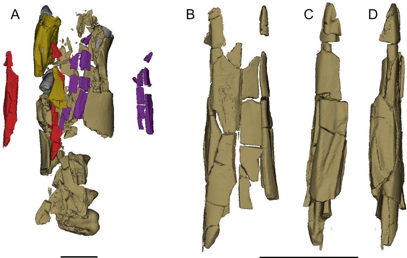
Figure 5. Restoration process for the nasal bone. A) Original specimen showing the in situ fragments of the left (in red) and right (in purple) nasal bones and the reconstruction of both on each side; B) virtual restoration of the joined left and right nasals; C-D) lateral views of the right and left nasals respectively. Scale bars = 1 cm.
