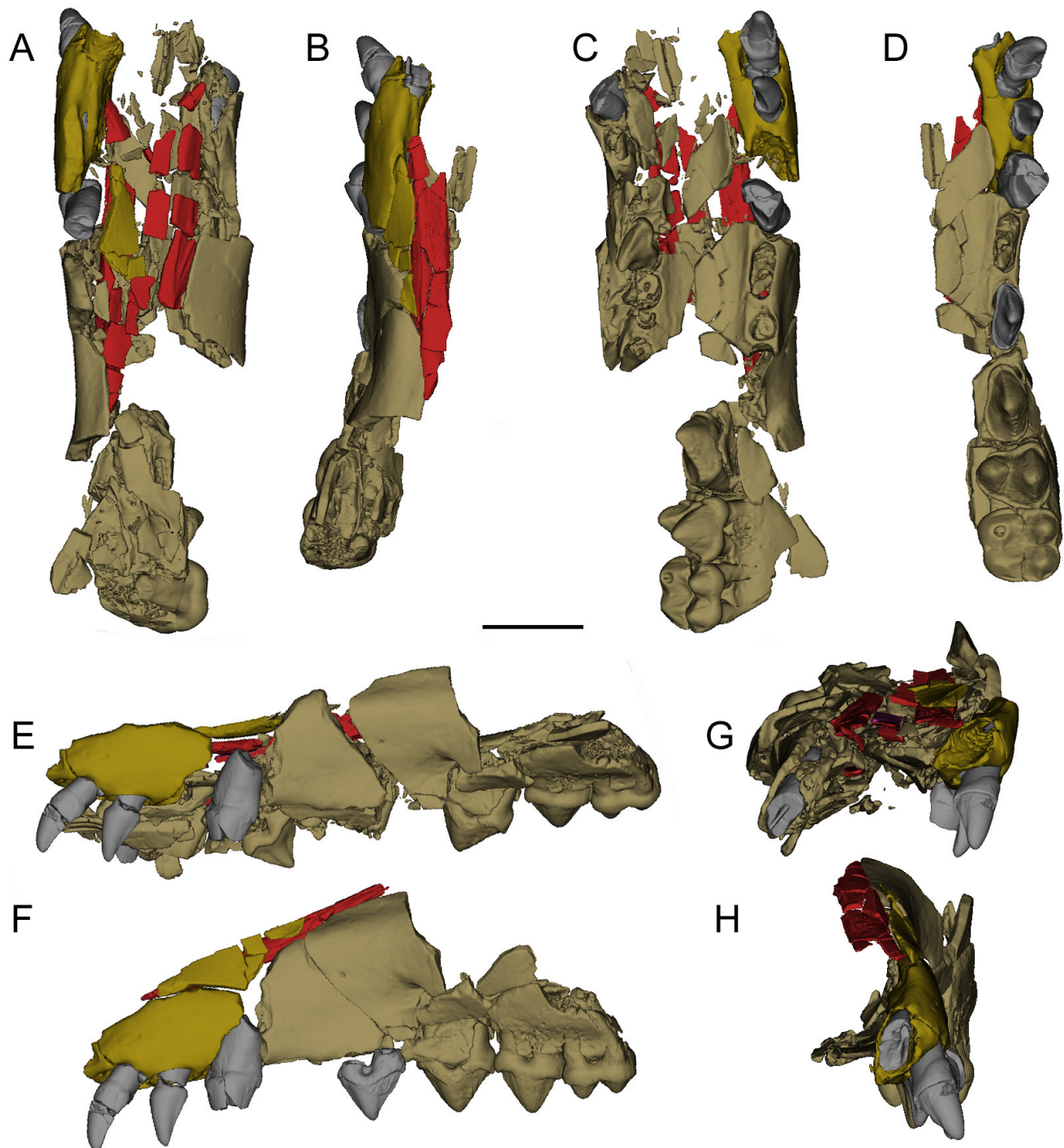
Figure 4. Restoration of the left side of the specimen GU/RJ/157; A, C, E, G, dorsal, ventral, left lateral and anterior views respectively showing the broken specimen; B, D, F, H, dorsal, ventral, left lateral and anterior views respectively showing the restored specimen. Premaxilla fragment appear in yellow, nasal fragments in red. The P2 was mirrored from the right side of the specimen where it is preserved. Scale bar = 1cm.
