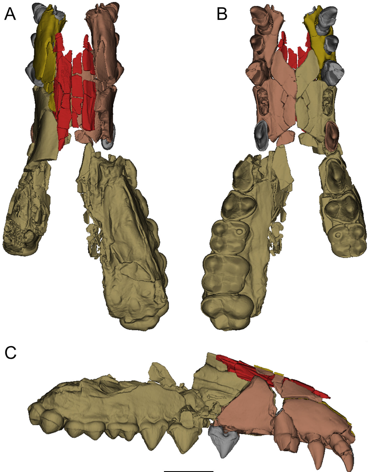
Figure 6. Tentative restoration of a "complete snout" using mirror meshes of the left part (in pink) and the large fragment of right maxilla bone. Scale bar = 1 cm.
