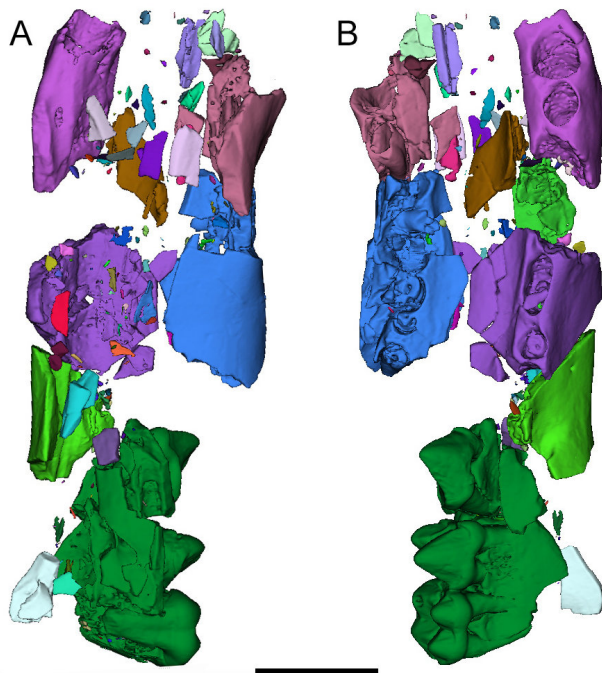
Figure 3. Illustration of the initial model in A) dorsal and B) ventral views showing the various non-contiguous parts that could be automatically separated as individual 3D objects using MorphoDig (Lebrun 2018, connectivity tool, decomposition, random colors); the anterior dentition and contiguous bone fragments were removed manually through segmentation process with the software Avizo Lite 9.3.0 ® (Thermo Fisher Scientific). Scale bar = 1cm.
