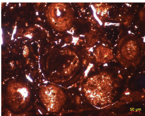
Fig. 2:3 – Sample CH02 exhibiting iron-rich glaebules cemented with secondary calcite (PPL).
