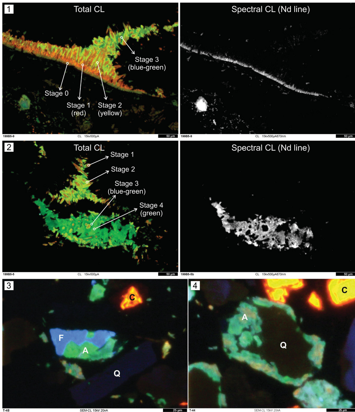
Fig. 2 – Cathodoluminescence imaging of apatite in the Saint-Ghislain ironstone. Photos 1 and 2 depict the diagenetic sequence in total (left) and spectral (right) CL (optical CL, scale bar 50 µm). The latter show the distribution of neodymium, which is not visible in total CL because it occurs in the near-infrared. In photos 3 and 4, apatite is replacing feldspars and quartz grains (SEM-CL, scale bar 25 µm). F = feldspar, Q = quartz, A = apatite and C = calcite.
