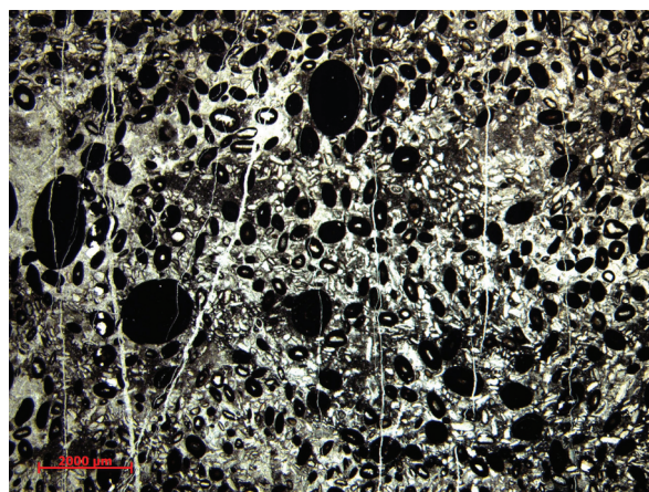
Fig. 22 – Sample Verviers VRD-27-2. Hodimont Formation. Distal facies. Hematitic ooids and micro-oncoids. Oolitic pack-to grain-ironstone. Micrograph of thin section in transmitted polarized light, without crossed polarizers.
