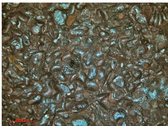
Fig. 8 – Emsian-Eifelian OIS, Heisdorf Formation, Hammermühle, Hillesheim (Germany). Coarse-grained, badly heterogenous hematitic OIS with ferruginized flattened bioclasts (“fossil ore”). Macroscopical view of rough surface.
