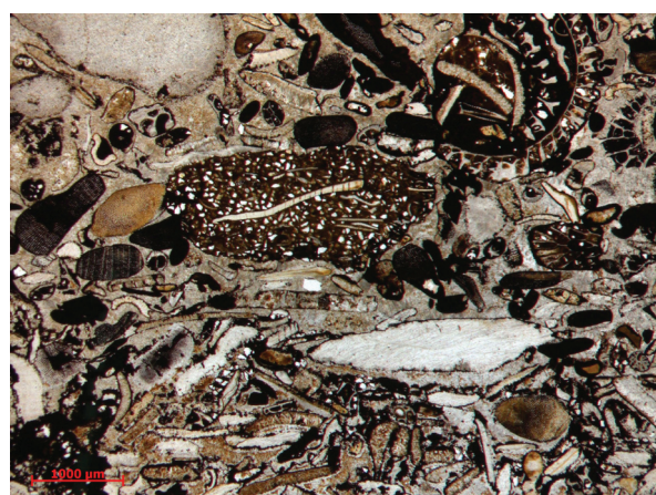
Fig. 16 – Oberahreck, sample OBA-01: Heisdorf Formation (Germany), bioclastic iron-grainstone with intraclasts and lithoclasts. Ferruginized bioclasts consists of crinoid ossicles, bryozoans, brachiopod shells, etc. Micrograph of thin section in transmitted polarized light, without crossed polarizers. Scale bar is 1 mm.
