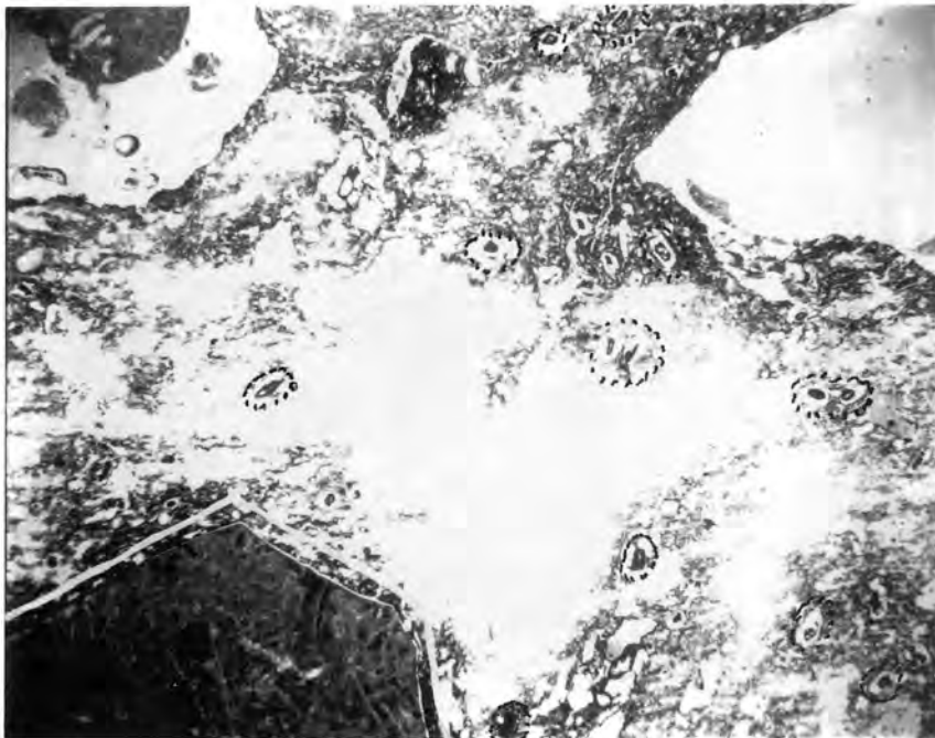
FIG. 55. — Microphoto of flint and plant-tempered ceramic ware. Vessel sherd B1-1-1, 20X
