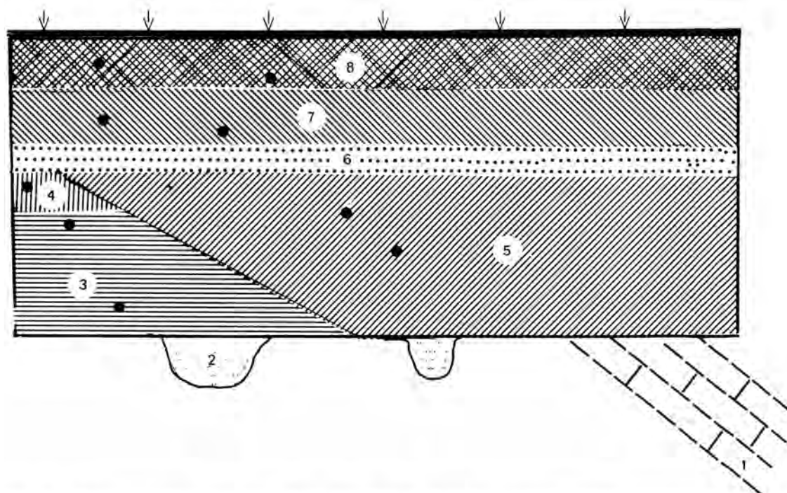
FIG. 59. — Ground profile at Le Clypot, Neufvilles, Hainaut, Belgium. 1 = Carboniferous limestone. 2 = Landenian sand with glauconite. 3 = Tertiary clay. 4 = Weathered top of Tertiary clay. 5 = Lower clay silt (≈ 50.000 B.P.). 6 = Sandy silt. 7 = Upper clayish silt (≈ 25.000 B.P.). 8 = Post glacial soil with B-horizon. (After a sketch by Prof. Dr. J. de Heinzelin). • = Clay samples.
