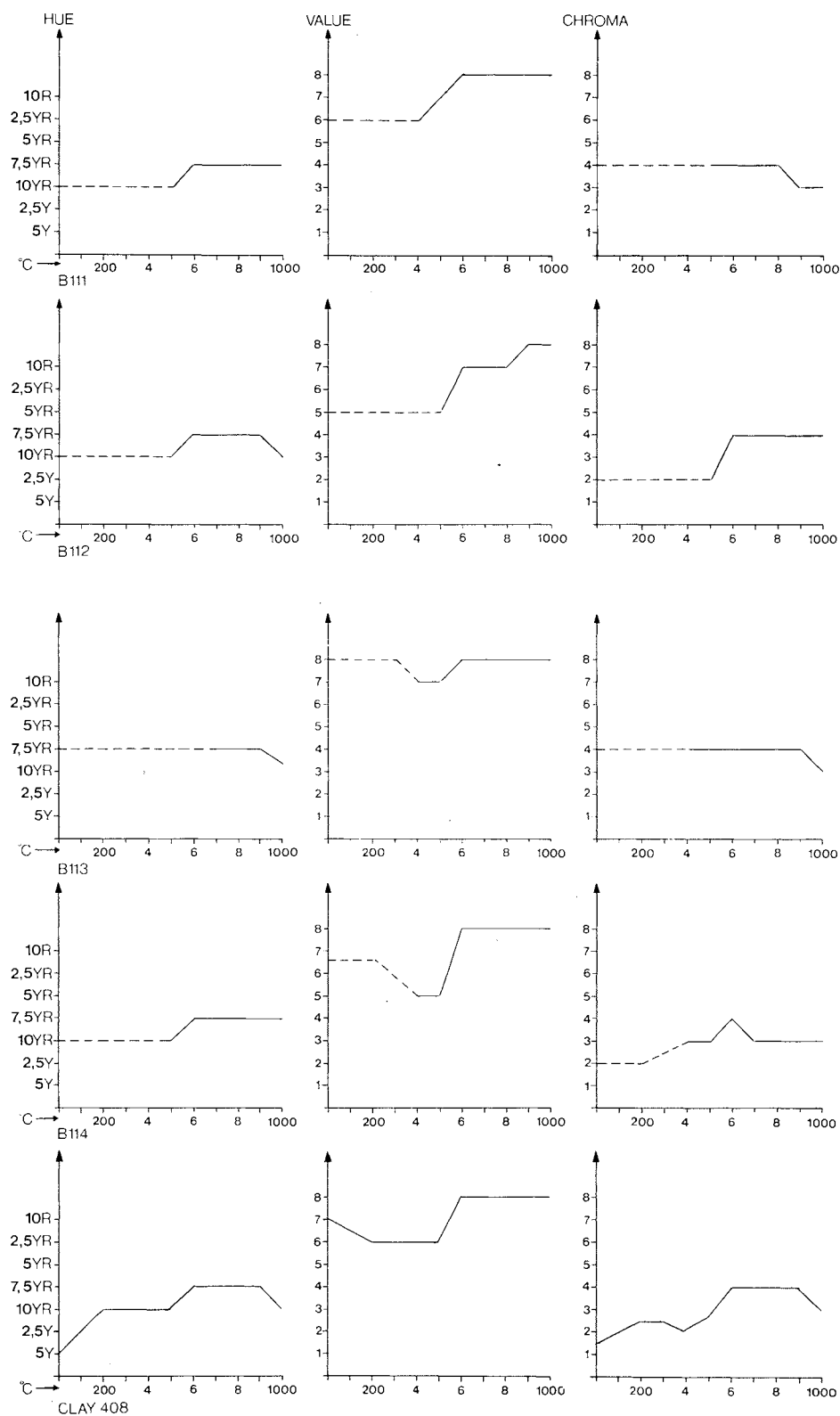
FIG. 61. — TCT-analysis
