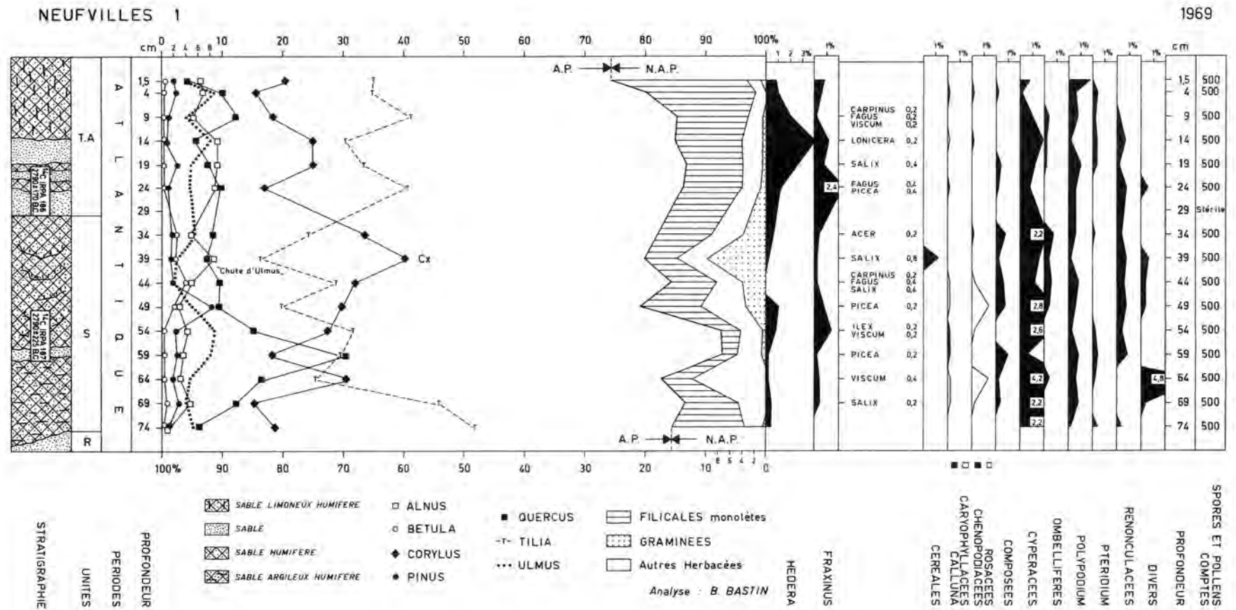
FIG. 12. — Diagramme pollinique NEUFVILLES 1 (B.B.).
