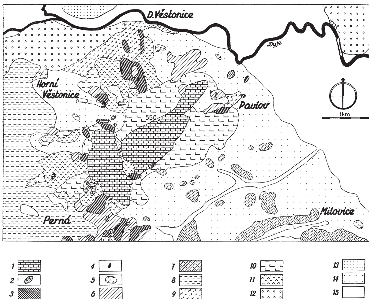
Fig. 3 – Geological map of the site area. 1: Jurassic limestone; 2: Cretaceous white marl; 3: Eocene/Lower Oligocene variegated silt; 4: Menilite slates; 5: Palaeogene conglomerate; 6: Middle Oligocene marl with sandstone; 7: Palaeogene sandstone; 8: Neogene calcareous silt and sandstone; 9- Pleistocene gray clay, in lower parts with sand; 10: Pleistocene loess enriched in debris; 11: Pleistocene calcareous debris on silt; 12: Pleistocene sandstone rubble; 13: Pleistocene eolian sands; 14: Pleistocene loess and loess clay; 15: Holocene sands and silts (after Klíma, 1963).
