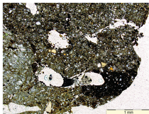
Fig. 5 – Marly, vesicular silt with embedded red powder (labeled in the text as “b”; lower hand-right quadrant) partially destroyed by microorganisms. Faecal pellet and bone fragments are visible (sample DVI 9, X nicols).
