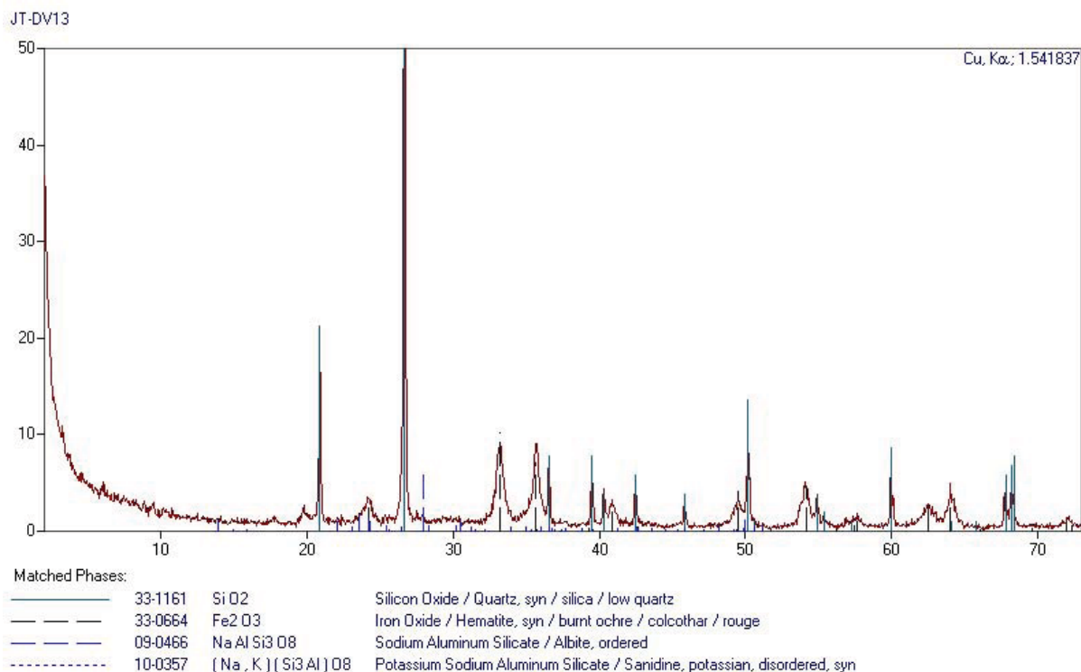
Fig. 21 – Diffractogram of the red lump, sample DVI 13 (Trąbska, 2015).
