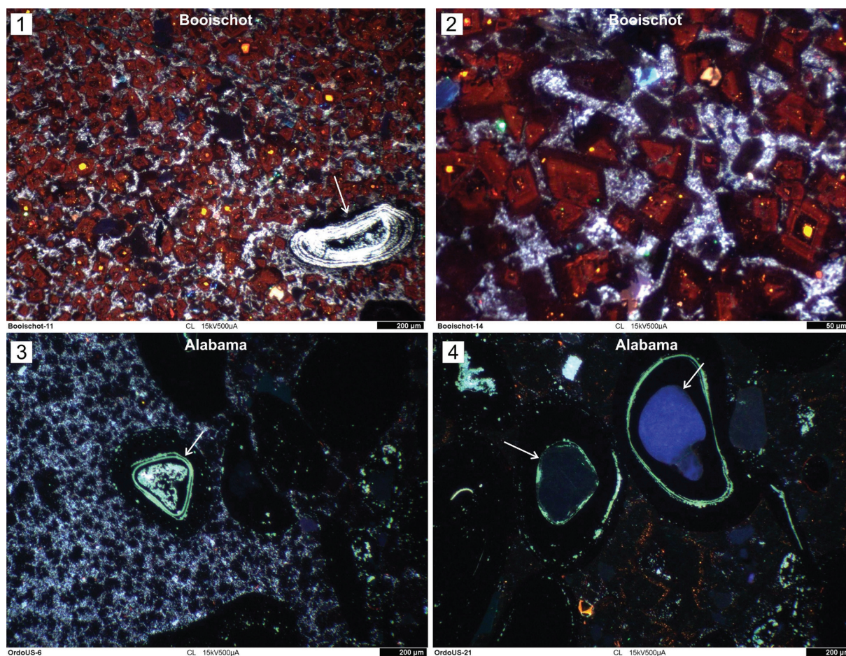
Fig. 4 – Cathodoluminescence imaging of selected Booischot (1-2) and Alabama (3-4) oolitic ironstone samples. In photo 1 apatite within the fine-grained groundmass and ooid laminae is white-luminescing. The close-up in photo 2 shows the details of the groundmass and the red-brown luminescing dolomite rhombs. Photos 3 and 4 depict the cathodofacies of the Alabama oolitic ironstone which comprises fine-grained groundmass apatite with non-luminescing carbonates (dark spots in 3). Light-green luminescing apatite occasionally occurs within the ooid laminae and the nucleus. Note the presence of well-rounded quartz grains as ooid nuclei (arrows in 4). Scale bars: 1-3 and 4 : 200 µm, 2 : 50 µm.
