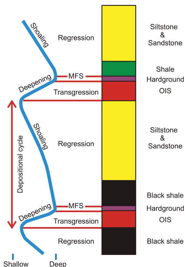
Fig. 2 – Generalised sequence-stratigraphical model for the Phanerozoic OIS (Bekker et al. , 2010).
