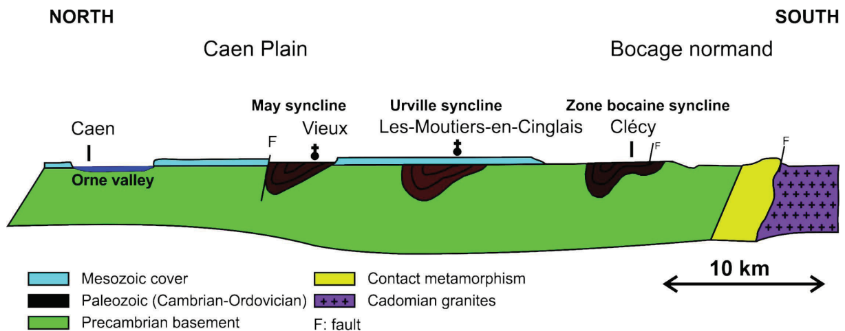
Fig. 14 – Geological cross-section through the Basse-Normandie.
