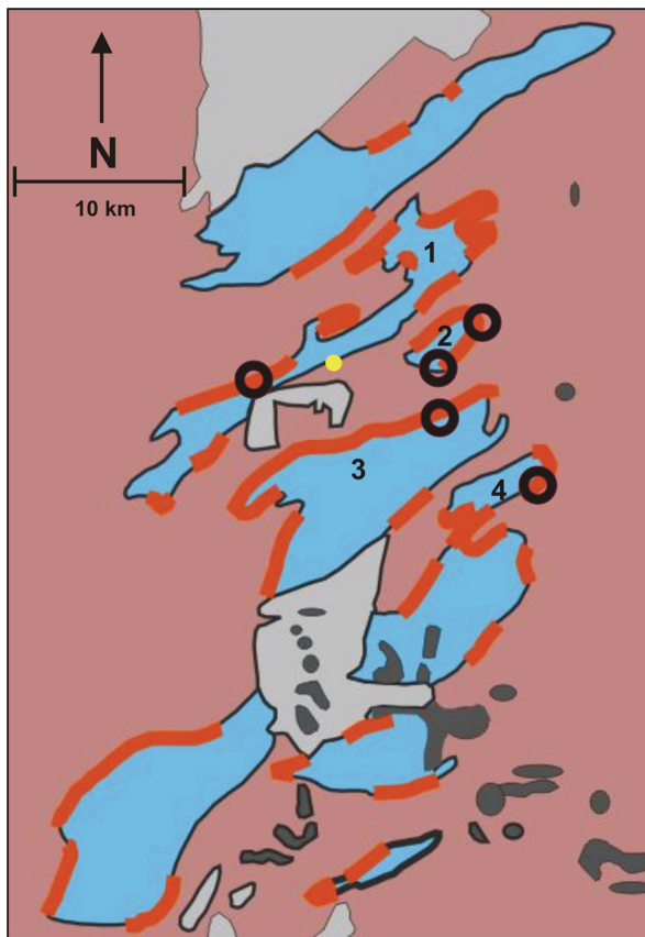
Fig. 4 – Detail of the previous geological map of the Eifel area, showing the location of the sampling points (open black circles). 1: Söthenicher syncline; 2: Rohrer syncline; 3: Dollendorfer syncline; 4: Ahrdorfer syncline. B: Blankenheim; D: Dollendorf; F: Freilingen R: Rohr; S: Stadt Kyll.
