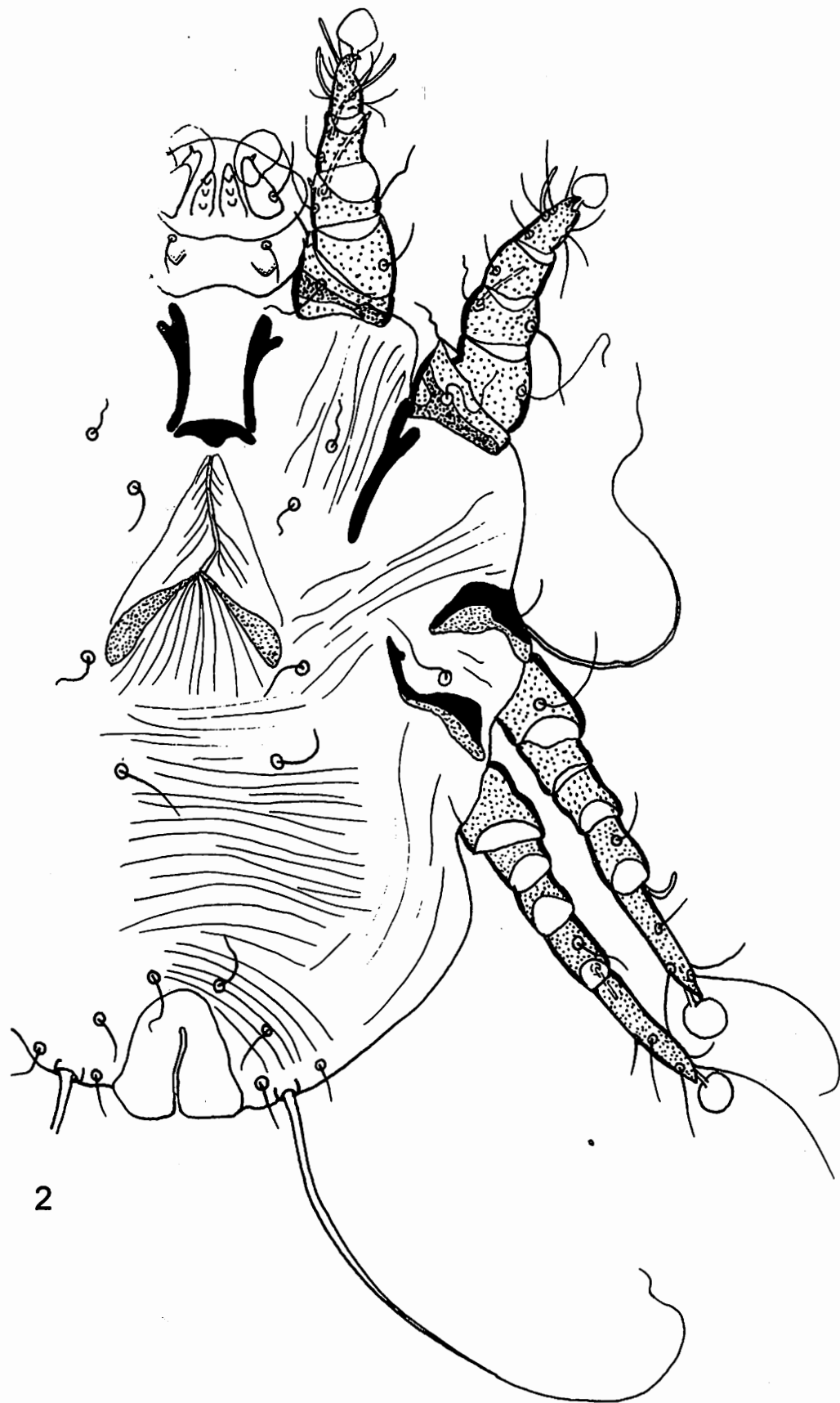
Fig 2. Female of Rallepidermoptes ralicola n. sp. in ventral view. Scale line 100 \mu m.
