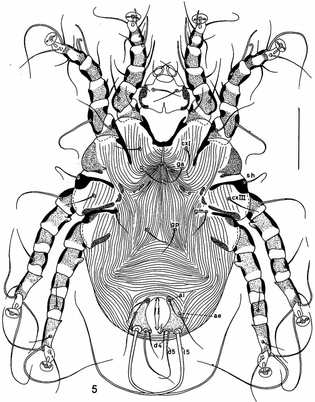
Fig. 5. Female of Passeroptes dermicola TROUSSERT in ventral view. Specimen from a sparrow from the Zoo of Antwerp. Scale line 0.05 mm (From FAIN, 1965: Fig. 141).
