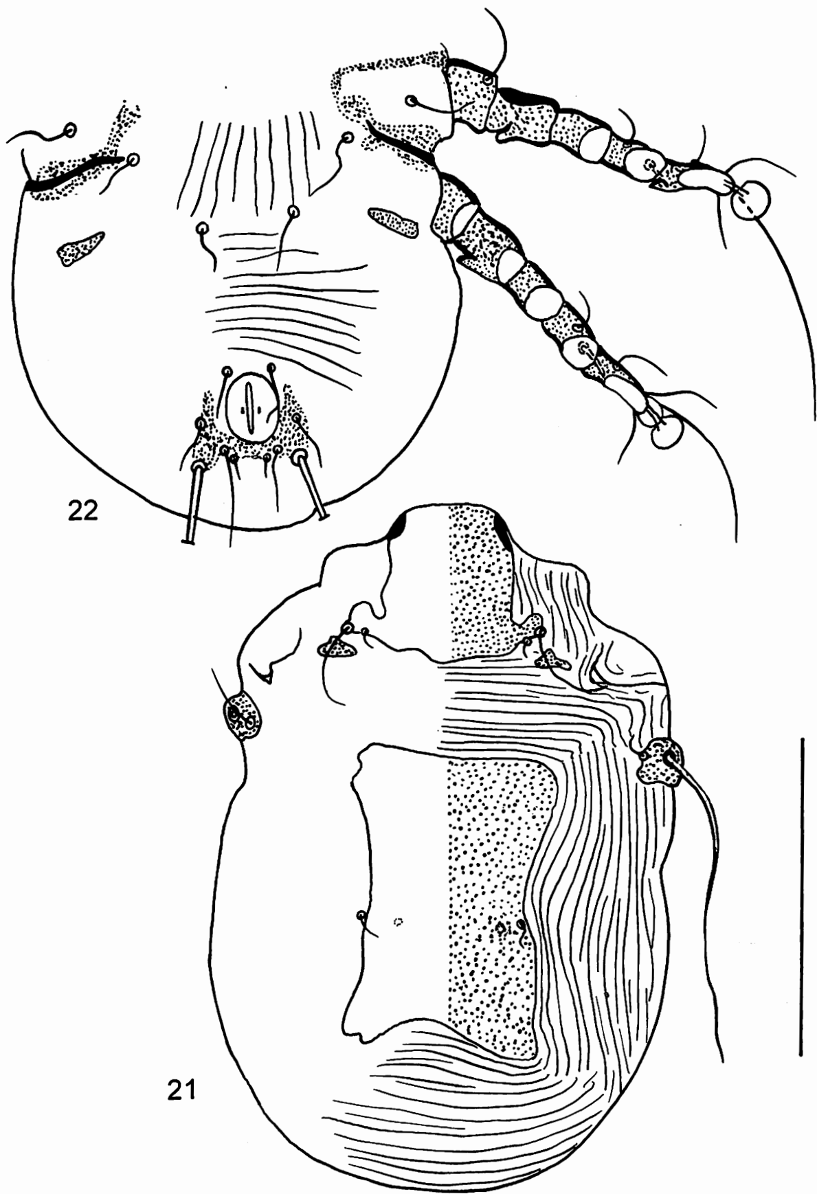
Figs 21-22. Female of Passeroptes ampeliceps n. sp. Dorsal view (21); opisthosoma in ventral view (22). Scale line 100 \mu m.
