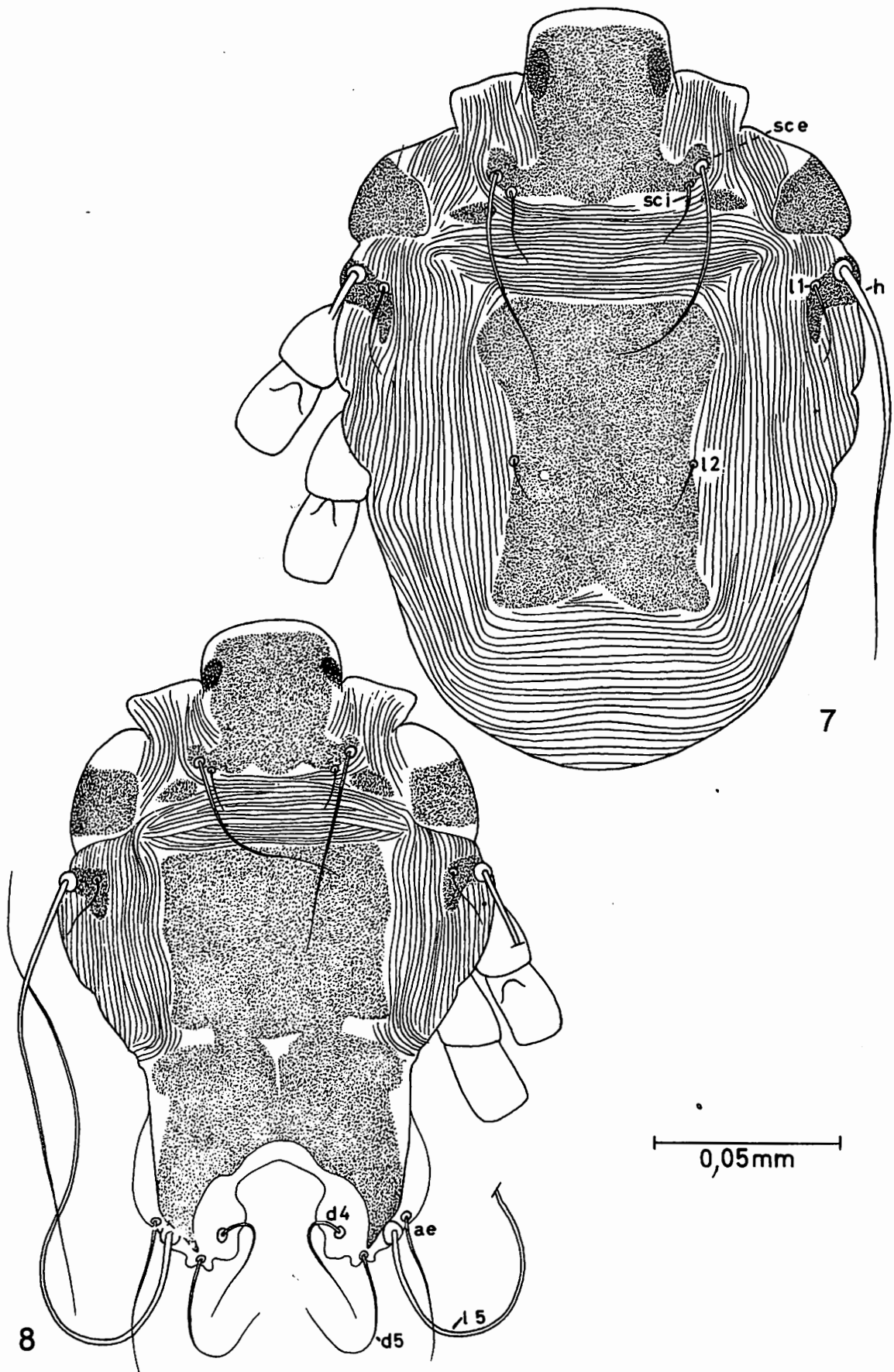
Figs. 7-8. Passeroptes dermicola TROUËSSART. Female in dorsal view (from a sparrow that died in the Zoo of Antwerp) (7); paralectotype male in dorsal view (8). Scale line 0.05 mm (From FAIN, 1965: Figs. 143 and 144).
