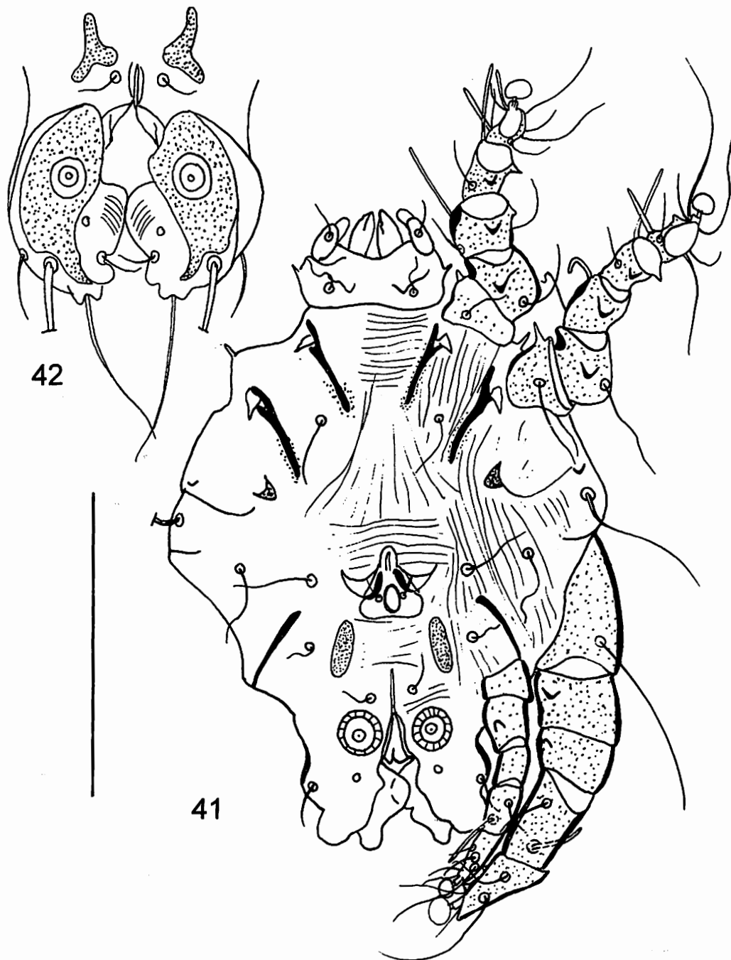
Figs 41-42. Males of Paradermation spp. P. colii in ventral view (41); opisthosomal lobes of P. intercalatum FAIN in ventral view (42). Scale lines 100 \mu m (Fig. 41) and 50 \mu m (Fig. 42).
