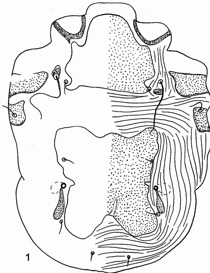
Fig 1. Female of Rallepidermoptes ralicola n. sp. in dorsal view. Scale line 100 \mu m.
