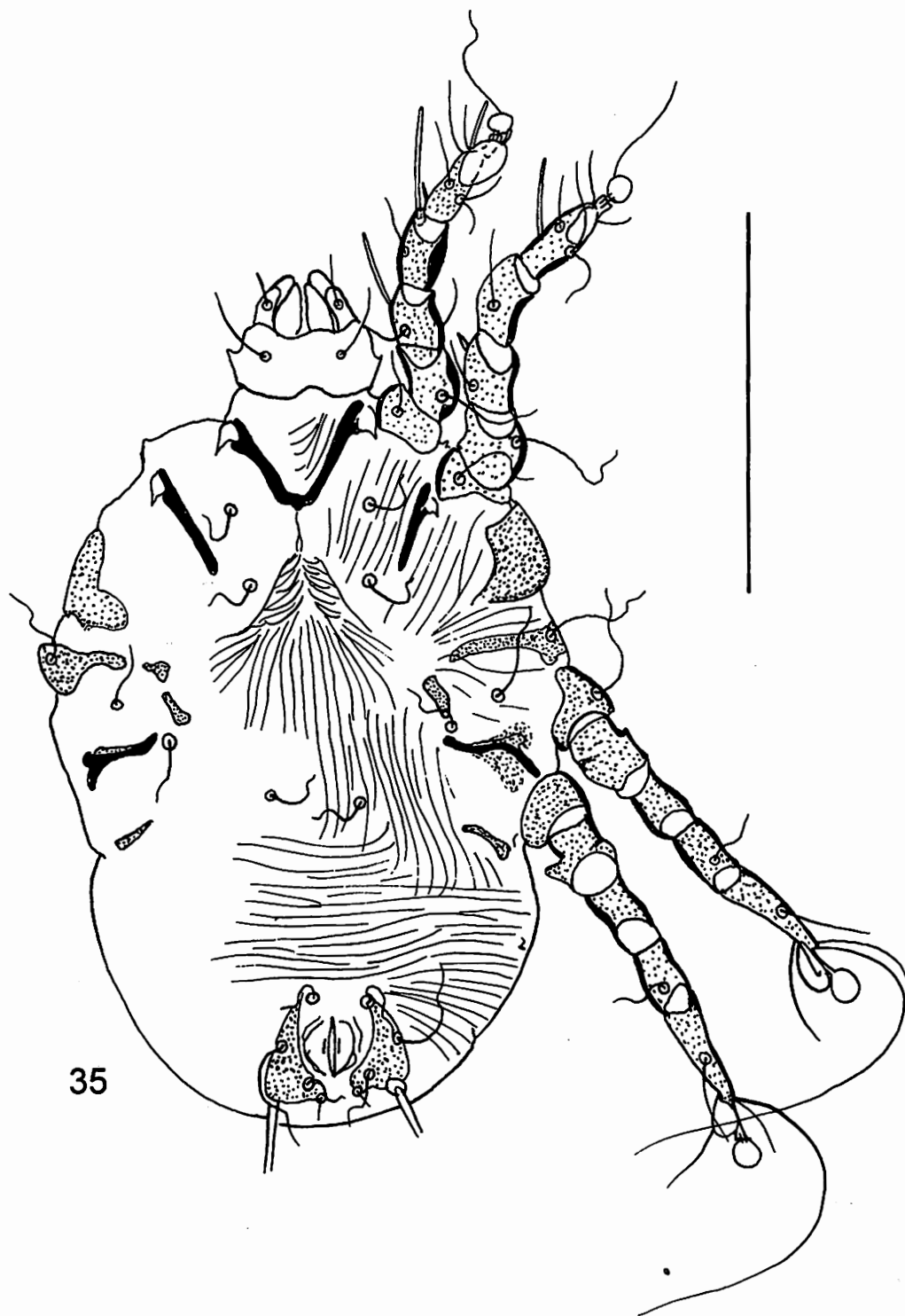
Fig. 35. Female of Passeroptes oeanthe n. sp. Ventral view. Scale line 100 \mu m.
