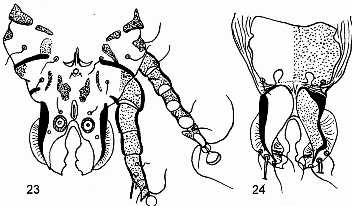
Figs 23-24. Male hysterosoma of Passeroptes amplicepts n. sp. Ventral view (23) and in dorsal view (24). Scale line 100 \mu m.
