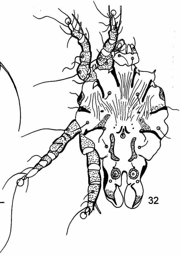
Figs 31-32. Male of Passeroptes hirundiphilus n. sp. Dorsal view (31); ventral view (32). Scale line 100 \mu m.
