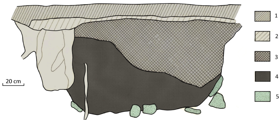
Fig. 3 – Cross-section of the presumed natural pit feature at the location of the former barrow n°82. Key: 1. Actual A-layer; 2. Disturbed layer; 3. 19th century trench; 4. Compact dark grey sandy fill; 5. In situ sandstones with capping.
