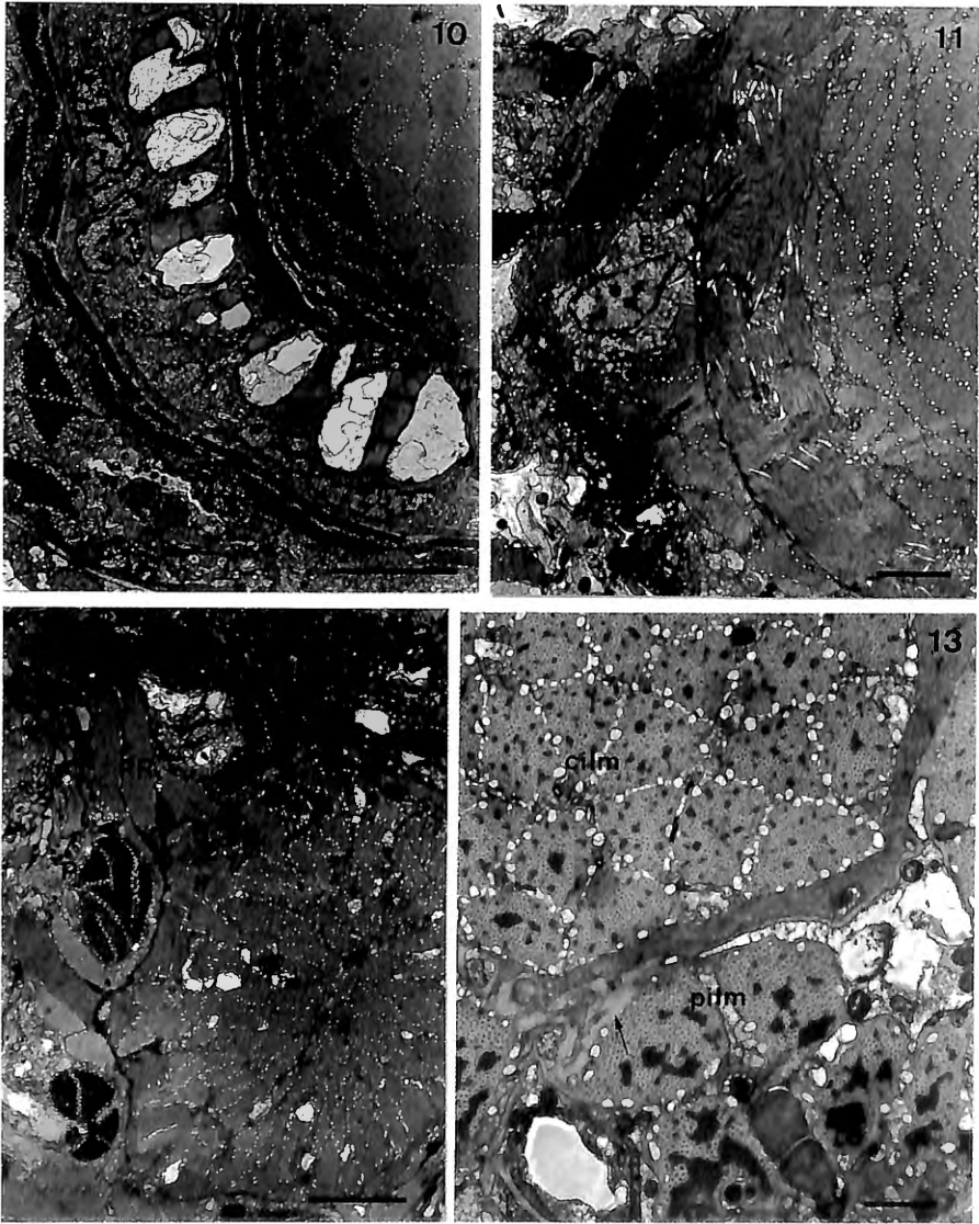
Figs 10-13. — Zonorhynchus seminascatus . — 10. Nucleo-glandular girdle with groups of g_1 and g_2 gland necks and nuclei of S_2 . Scale bar: 5 \mu\text{m} . — 11. Cross section of the median part of the bulb with insunk nucleated cell part of B in between proboscis retractors ( PR ). Scale bar: 2 \mu\text{m} . — 12. Cross section of the posterior part of the bulb with proboscis retractors ( PR ) and protractors ( P ). Scale bar: 5 \mu\text{m} . — 13. Cross section in the cone with central cylinder ( cilm ) and peripheral longitudinal muscles ( pilm ), separated by a circular muscle fibre. Note the ECM (arrow). Scale bar: 1 \mu\text{m} .
