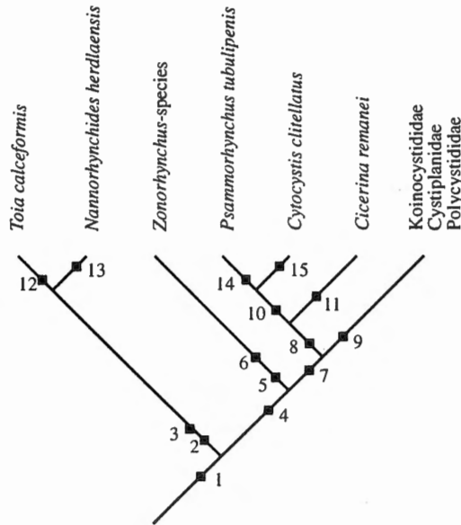
Fig. 14. – Tentative cladogram mainly based on characters derived from ultrastructural investigations on the proboscis of eukalyptorhynch species investigated. See text for the description of the apomorphic characters 1 to 15.
