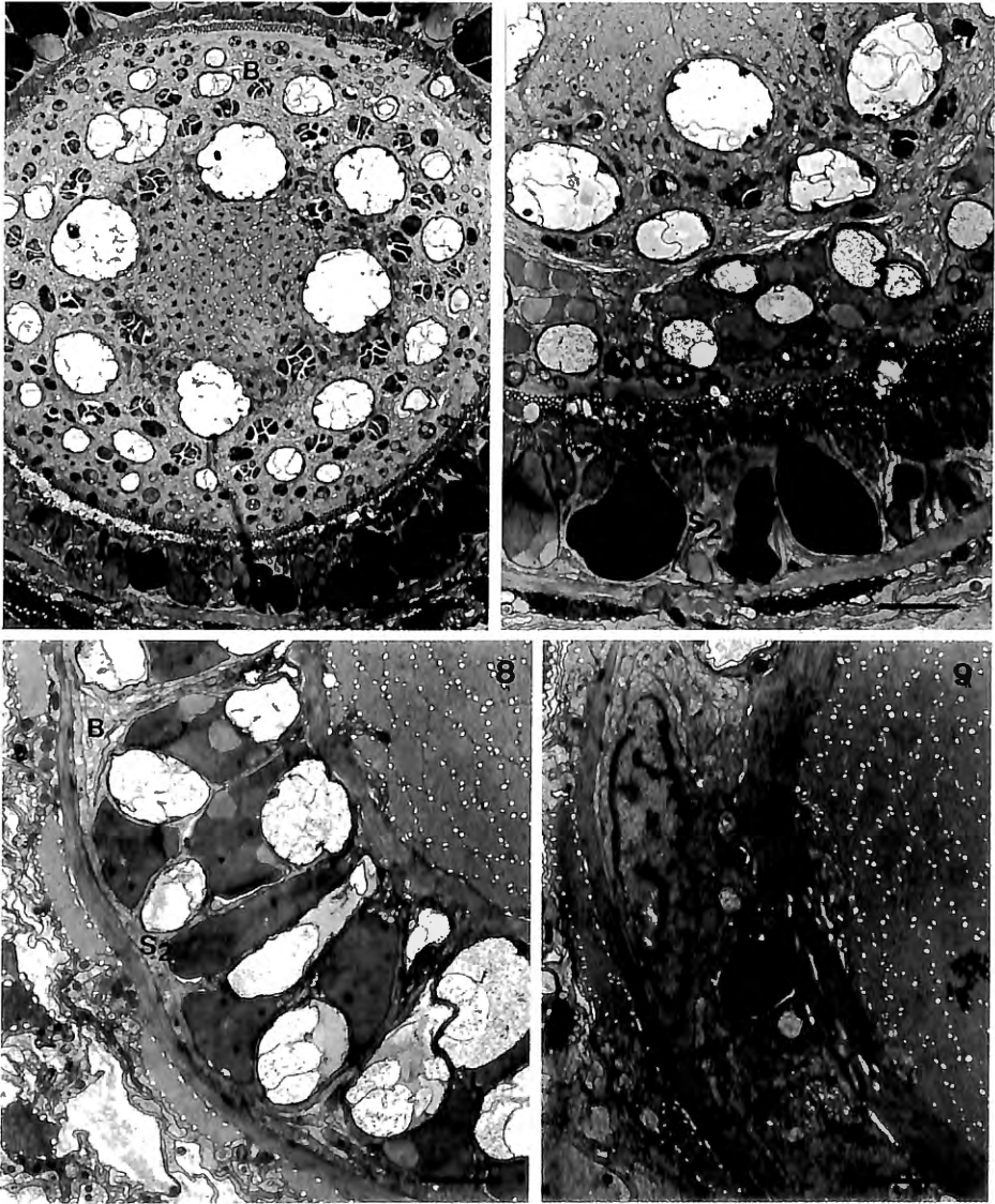
Figs 6-9. - Zonorhynchus sp. - 6. Cross section of the cone clearly showing alternating g_8 and g_9 gland necks with in between g_8 and g_{10} gland necks. Scale bar: 5 \mu m. - 7. Proximal belt of the sheath epithelium with g_7 , g_8 , and g_9 gland necks, basal cone epithelium with groups of g_8 and g_9 gland necks, and g_7 necks in the bulb. Scale bar: 2 \mu m. - 8. Cross section of the nucleo-glandular girdle showing type g_8 and g_9 gland necks and cytoplasmic cell parts of S_1 and B . Scale bar: 2 \mu m. - 9. Posterior portion of the nucleo-glandular girdle with nucleus of S_1 and cell strands of B . Scale bar: 2 \mu m.
