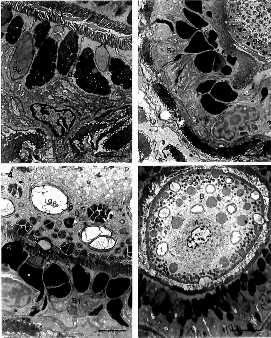
Figs 2-5. — 2. Z. seminascatus . Cells of the distal belt ( S ) with nucleus and g 1 and g 2 gland necks. Scale bar: 2 μm. — 3. Z. seminascatus . Distal belt of the sheath epithelium ( S ) surrounded by circular and longitudinal muscles, and apical cone epithelium ( A ) with g 1 gland necks. Scale bar: 2 μm. — 4. Zonorhynchus sp. Distal belt of the sheath epithelium ( S ), and basal cone epithelium ( B ) with g 1 and g 2 gland necks. Scale bar: 2 μm. — 5. Z. seminascatus . Cross section of the cone with nucleus of the apical cone epithelium ( A ), and basal cone epithelium ( B ) with alternating g 1 and g 2 gland necks. Scale bar: 5 μm.
