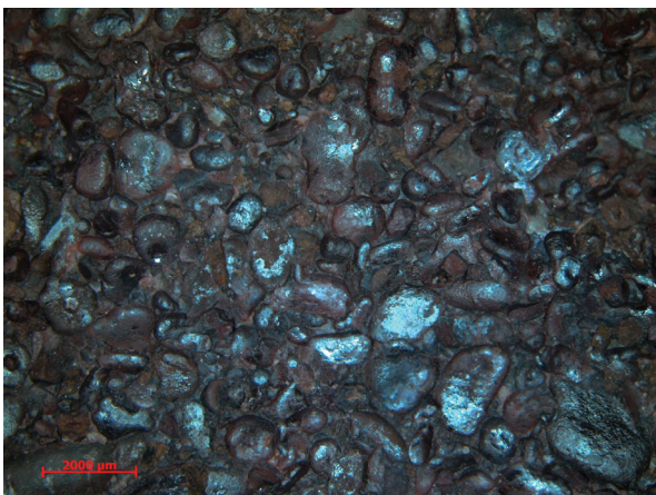
Fig. 9 – Emsian-Eifelian OIS, Heisdorf Formation, Hammermühle, Hillesheim (Germany). Detail of previous photograph: flattened and rounded ferruginized (hematitic) bioclasts. Scale bar is 2000 µm.
