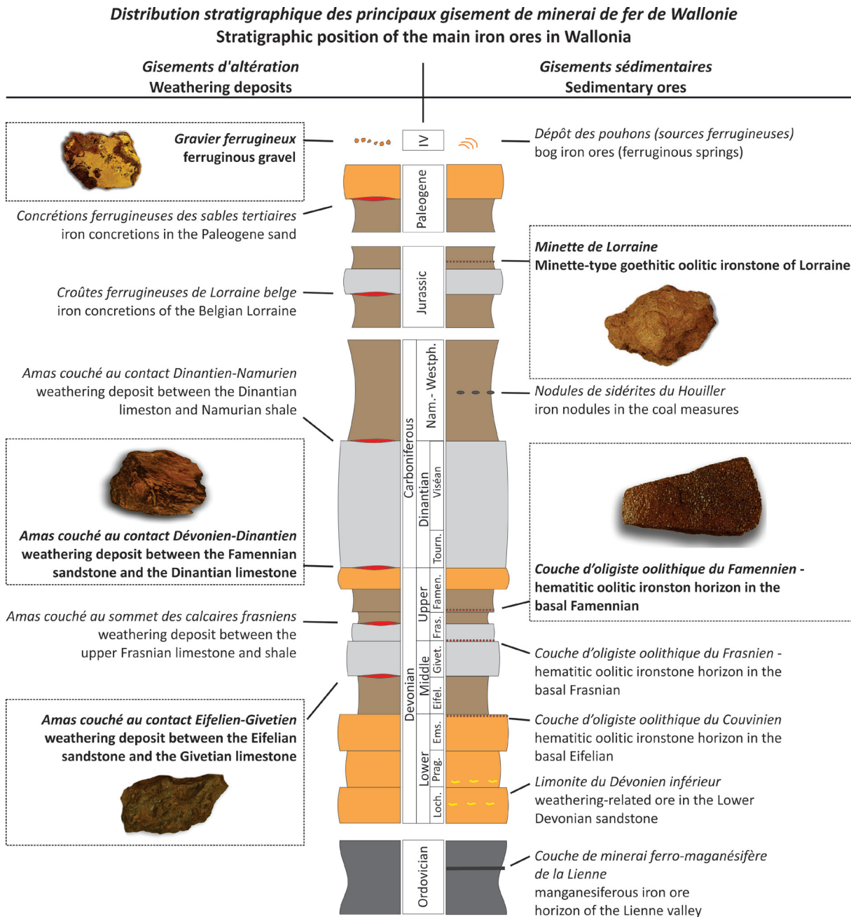
Fig. 2 – Stratigraphic position of the main sedimentary rocks-related iron ores of Wallonia. Illustrated ores (boxes) were the most important from an industrial and economical point of view. Fragments of ores c. 10 cm. Abbreviations: Loch. Lochkovian, Prag.: Pragian, Ems.: Emsian, Eifel.: Eifelian, Givet.: Givetian, Frasn.: Frasnian, Famenn.: Famennian, Tourn.: Tournaisian, IV: Quaternary.
