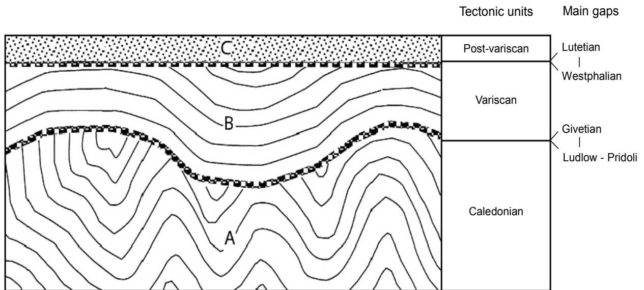
Figure 6. Synthetic sketch of the geometric relations between the tectonic units exposed along the Orneau Valley, where the main orogenic angular unconformities (A) and sedimentary gaps are summarised.
