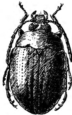
Stilbocistela manoiensis nov. sp. \times 7 .
