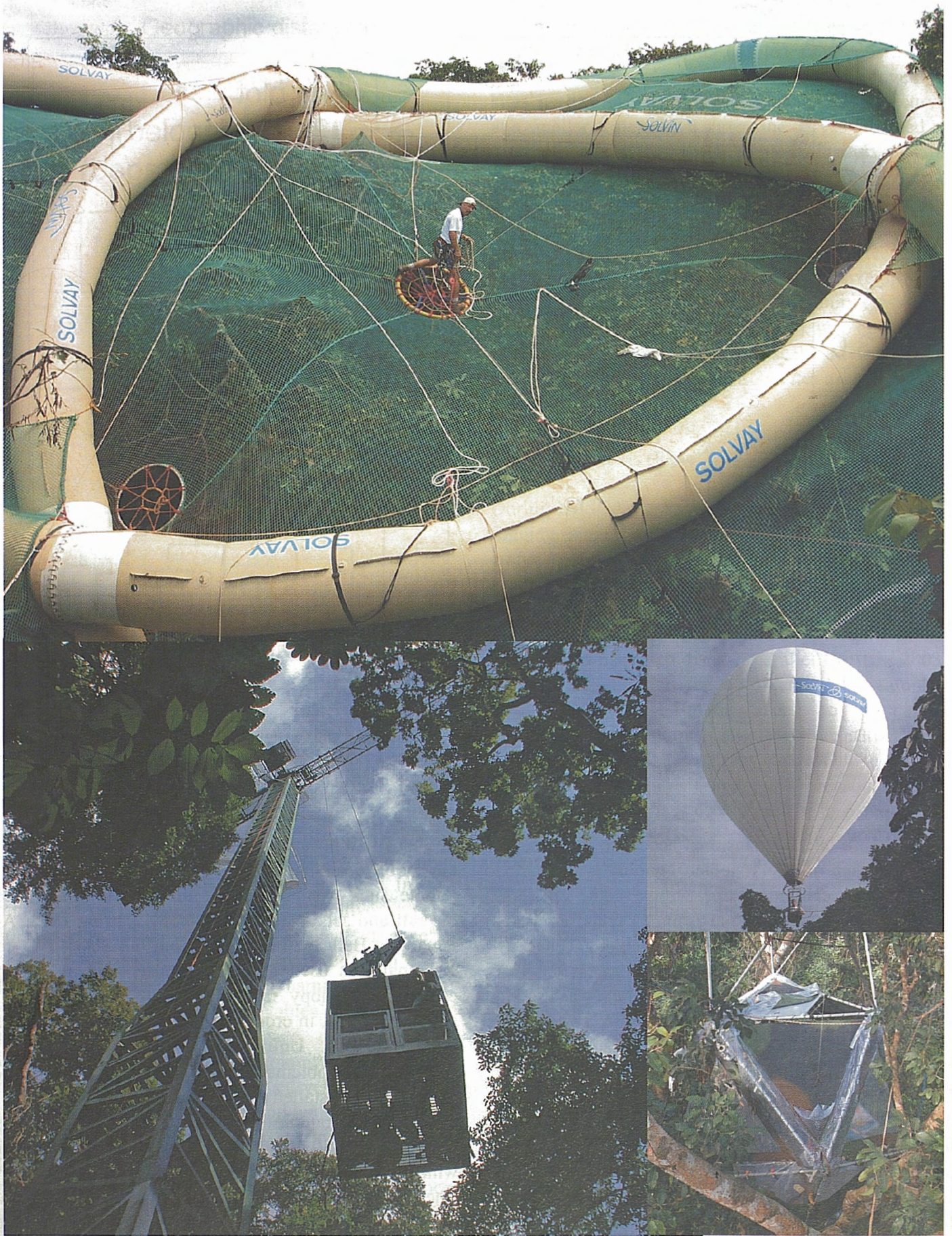
Plate 2 — Canopy access devices, clockwise: SolVin-Bretzel canopy raft, canopy bubble, Ikos tree house and canopy crane. Photos: S. Bechet, R. Le Guen, JO, ML.
