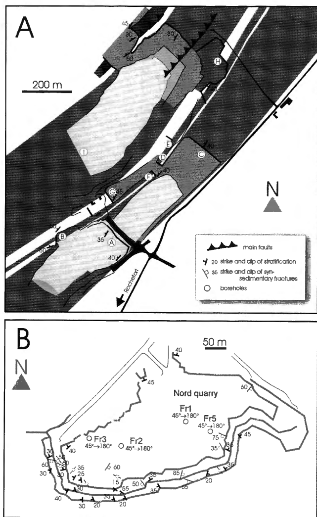
Fig. 3 — A. Location of sections B, D, E, F, G and H in the La Boverie quarry at Rochefort. B. Location of FR1-5 boreholes drilled in the Nord quarry at Frasnès; structural data are from BOULVAIN & COEN-AUBERT (1998).
