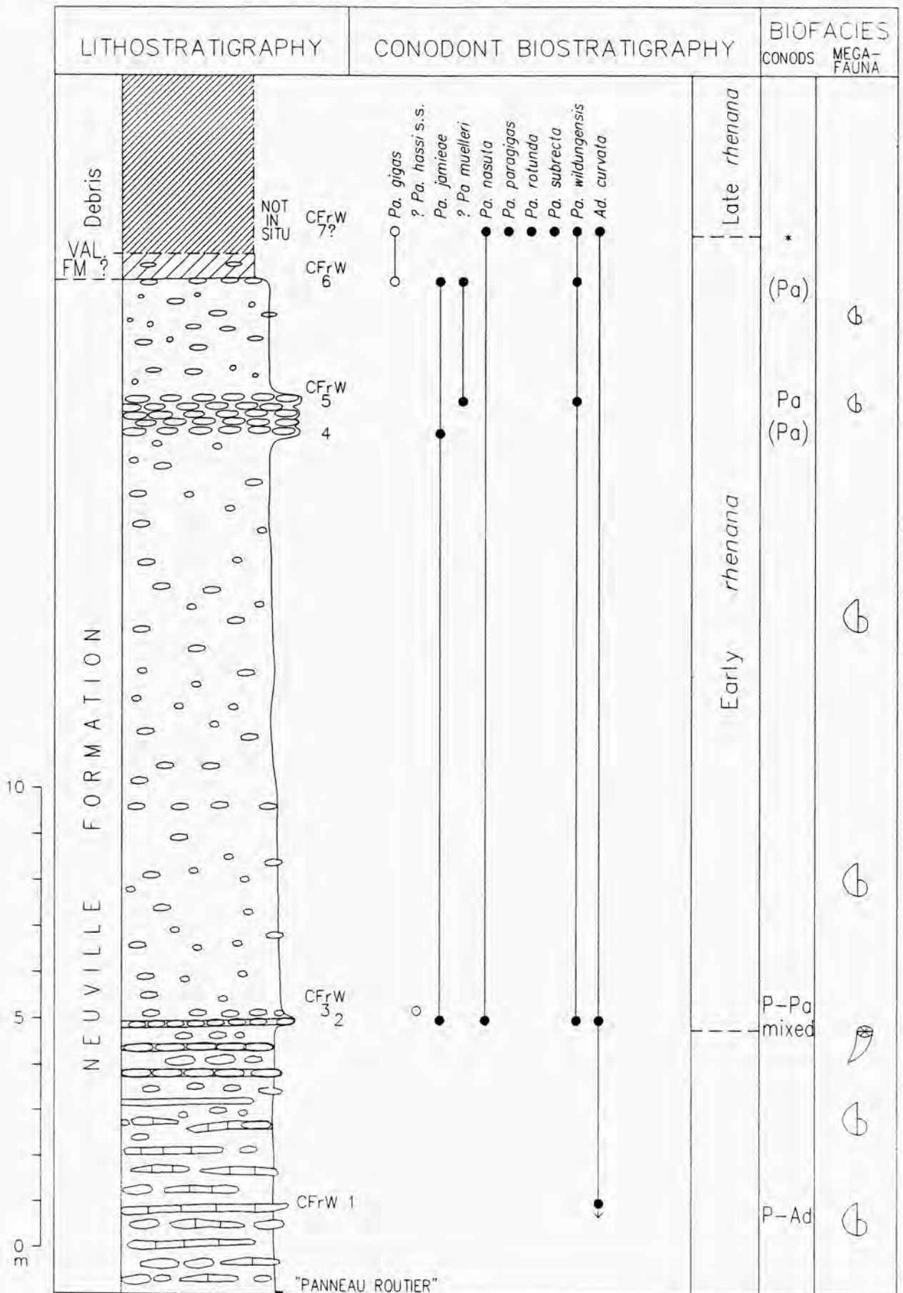
Fig. 4 - Stratigraphy and biofacies of the Frasnian-Wenlock section (CFrW).
