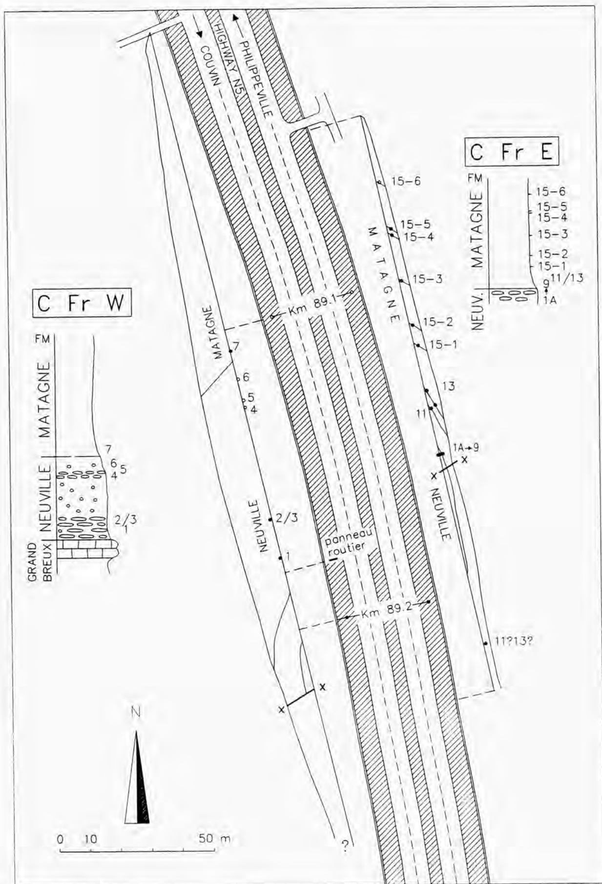
Fig. 3 – Location of the Frasnian sections (C Fr W, C Fr E).
