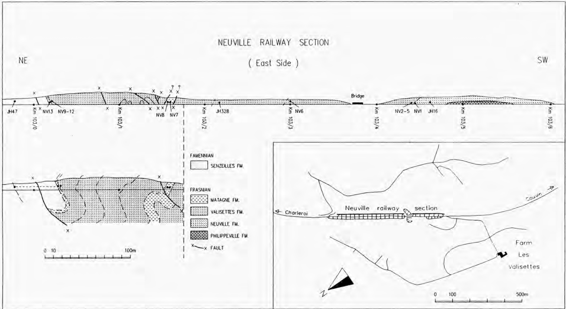
Fig. 10 – Location and sketch of the Neuville section (NV).
