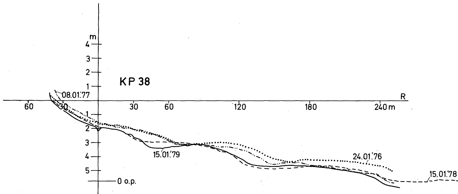
Fig. 2 - Station KP 38 (Klemskerke) Transversal profiles of the natural beach. Residual evolution during the period january 1976-january 1979. General lowering of the beach, progressing gradually away from the low water mark. Retreat of the wave exposed parts of the beach ridges. The terraced zone is less altered due to supply of dune sands.
