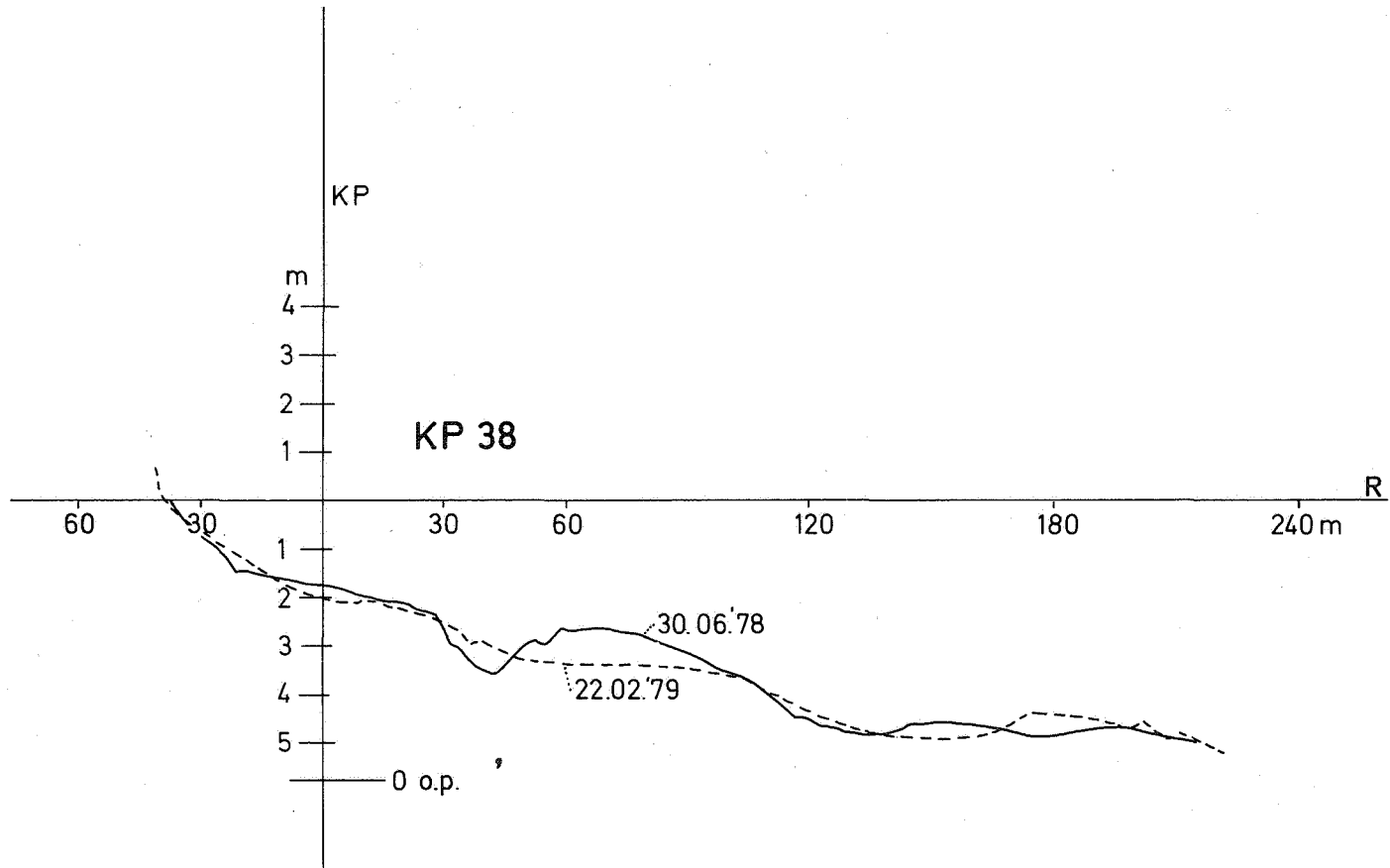
Fig. 1 - Station KP 38 (Klemskerke) Transversal profiles of the natural beach. Micromorphological difference between summer and winter beach.
